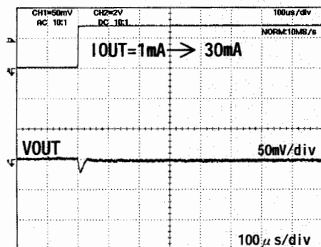
Fig.17 Load Transient response (Co=10 μF)
