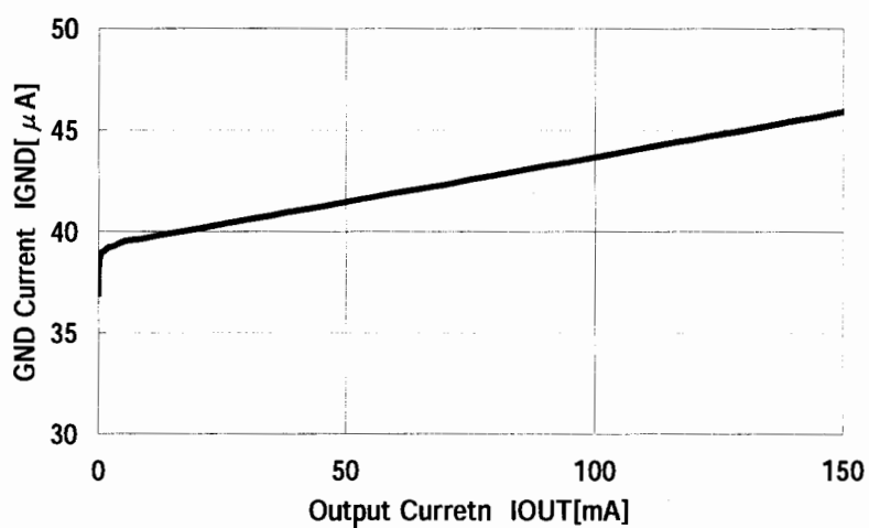
Fig.12 GND Current-Output Current
