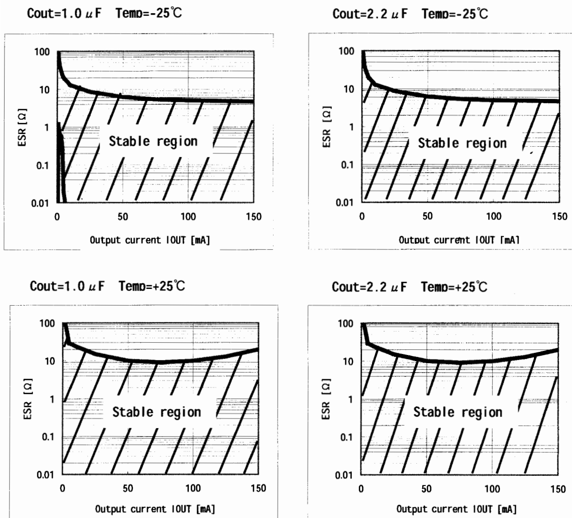
Fig.24 Stable region characteristic (Reference)
