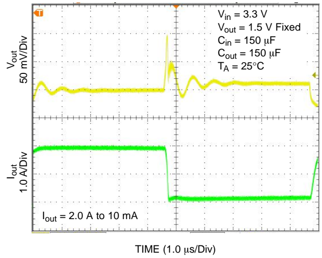
Figure 17. Load Transient Response
