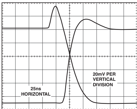
TPC 19. Magnitude Output Response to 4 dB Step, for P_{INPB} = -30 \text{ dBm} , P_{INPA} = -32 \text{ dBm} to -28 \text{ dBm} , Frequency 1900 MHz, No Filter Capacitor
