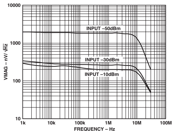
TPC 22. Magnitude Output Noise Spectral Density, P_{INPA} = P_{INPB} = -10 \text{ dBm} , -30 \text{ dBm} , -50 \text{ dBm} , No Filter Capacitor
