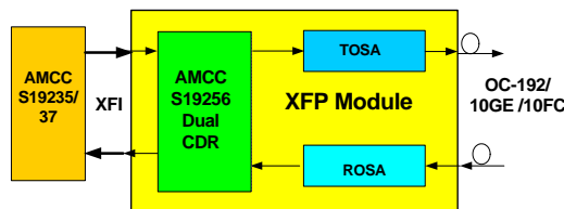
10 Gbps Line Card
