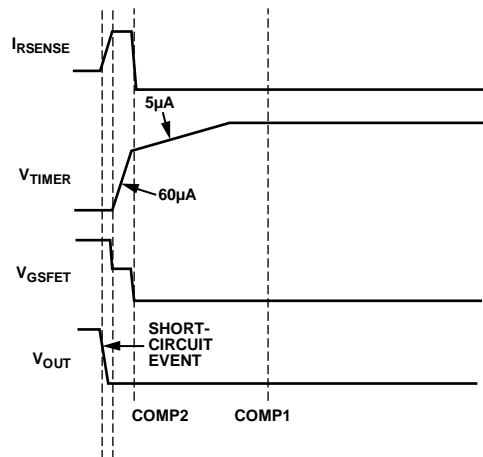
Figure 36. ADM1170-2 Latch Off After Overcurrent Fault
