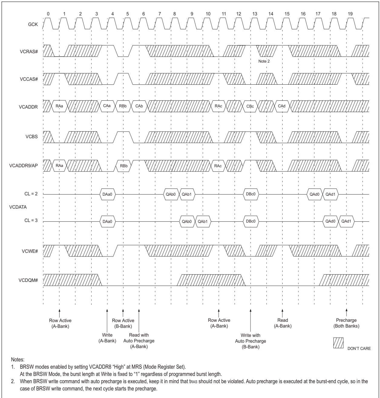
FIGURE 14 – SDRAM BURST READ SINGLE BIT WRITE CYCLE @ BURST LENGTH = 2
