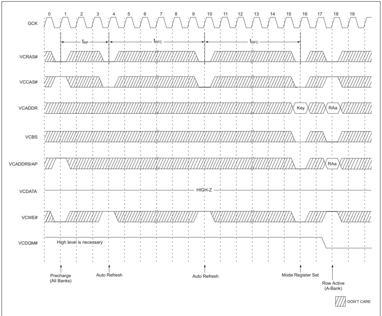
FIGURE 5 – SDRAM POWER UP SEQUENCE
