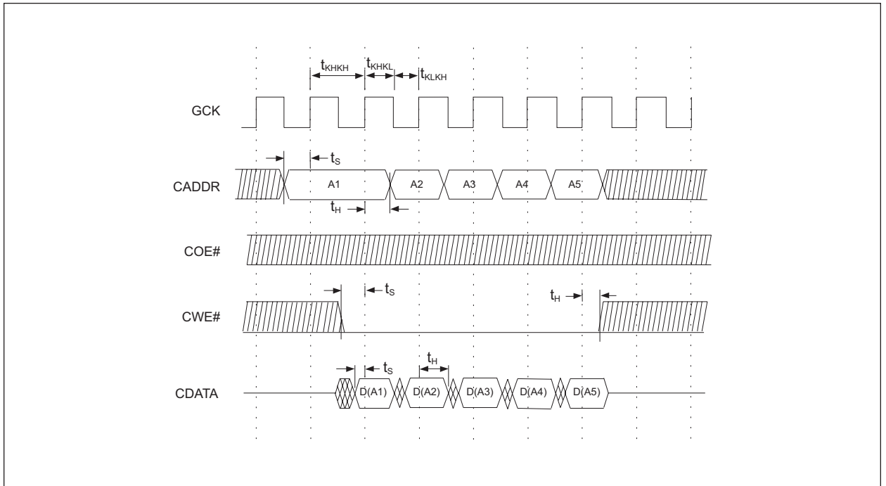
FIGURE 3 – SSRAM WRITE TIMING
