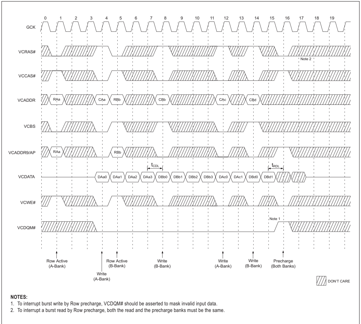
FIGURE 9 – SDRAM PAGE WRITE CYCLE AT DIFFERENT BANK @ BURST LENGTH = 4
