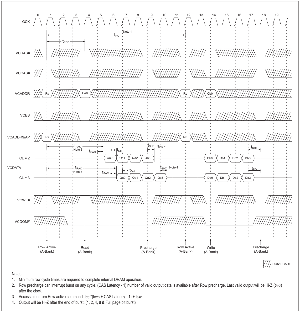
FIGURE 6 – SDRAM READ & WRITE CYCLE AT SAME BANK @ BURST LENGTH = 4
