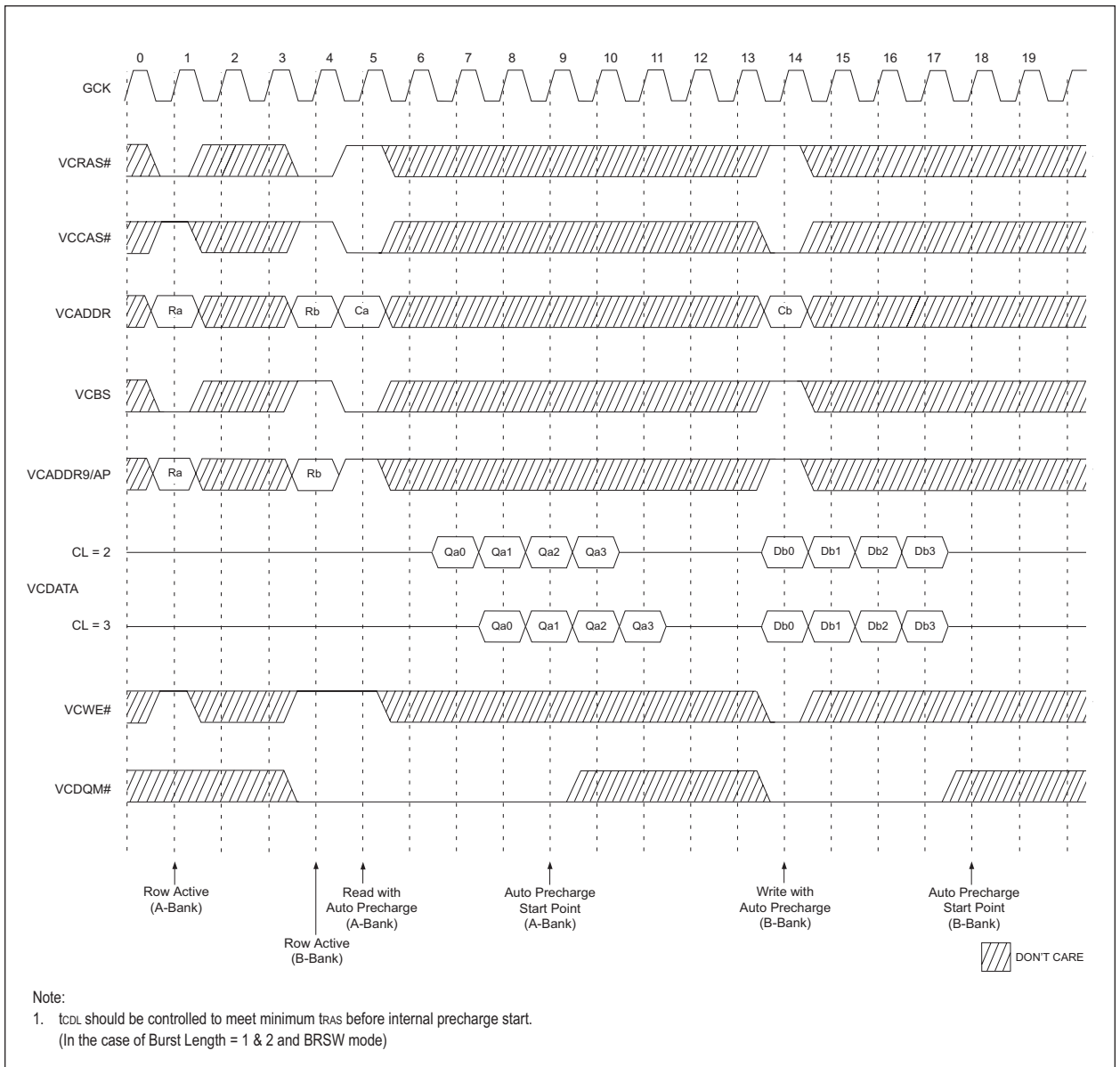
FIGURE 11 – SDRAM READ & WRITE CYCLE WITH AUTO PRECHARGE @BURST LENGTH = 4
