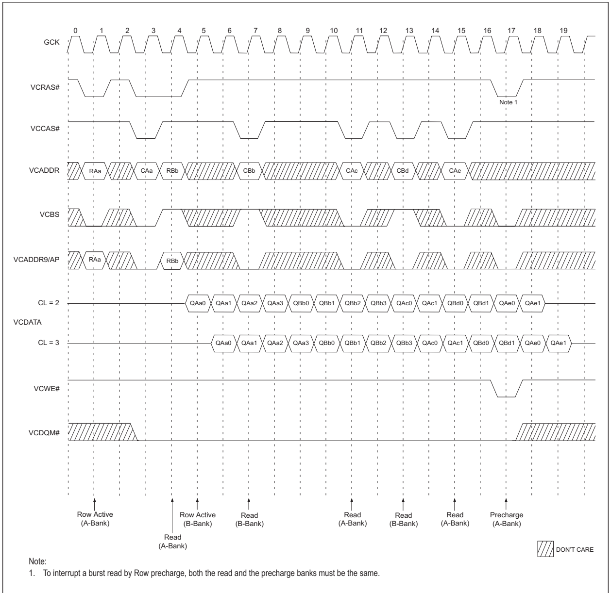
FIGURE 8 – SDRAM PAGE READ CYCLE AT DIFFERENT BANK @ BURST LENGTH = 4
