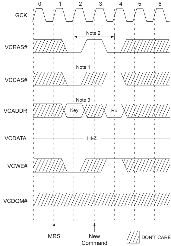
FIGURE 15 – SDRAM MODE REGISTER SET CYCLE
