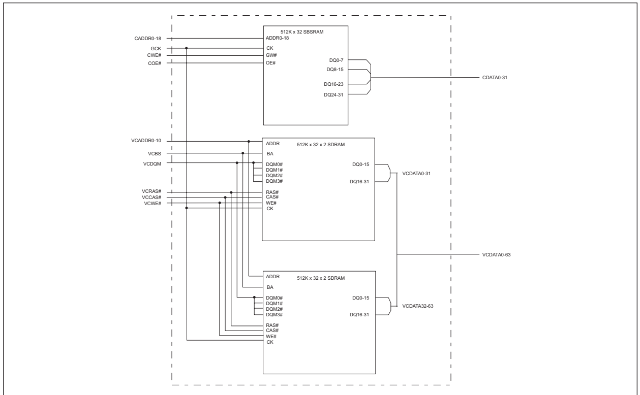
FIGURE 1 – BLOCK DIAGRAM 512K X 32 SSRAM / 1M X 64
