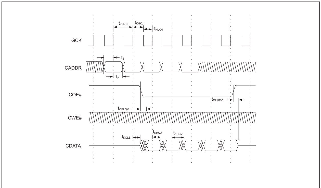
FIGURE 2 – SSRAM READ TIMING
