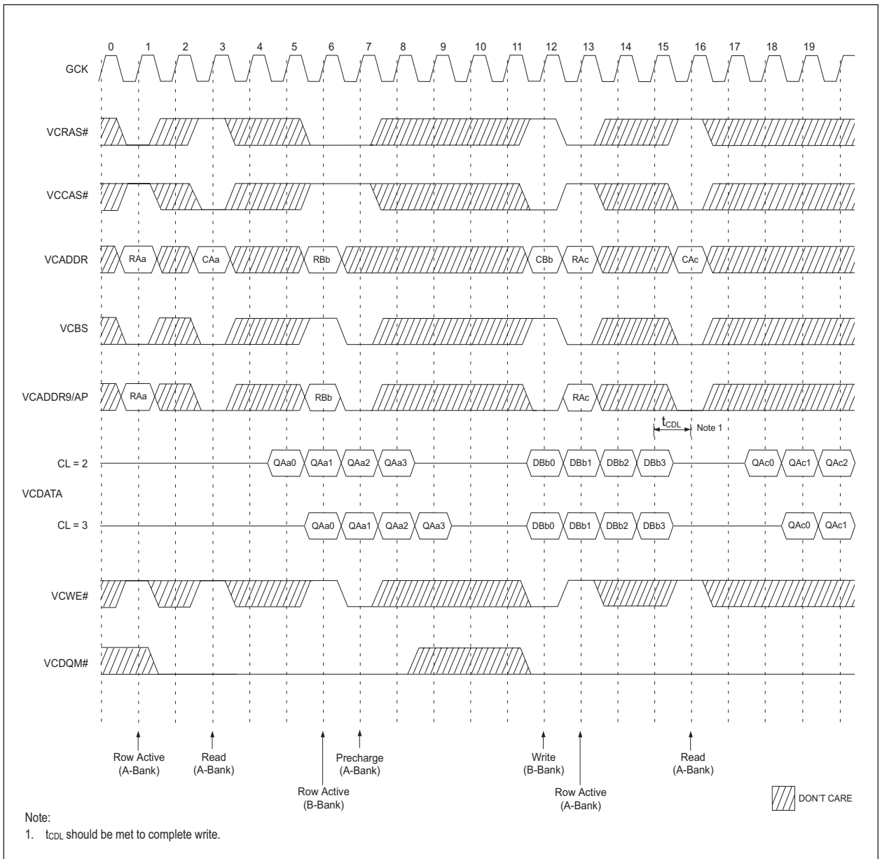
FIGURE 10 – SDRAM READ & WRITE CYCLE AT DIFFERENT BANK @ BURST LENGTH = 4
