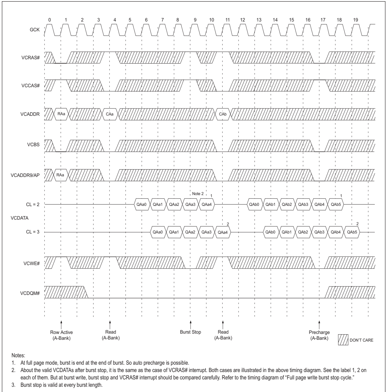
FIGURE 12 – SDRAM READ INTERRUPTED BY PRECHARGE COMMAND & READ BURST STOP @ BURST LENGTH = FULL PAGE
