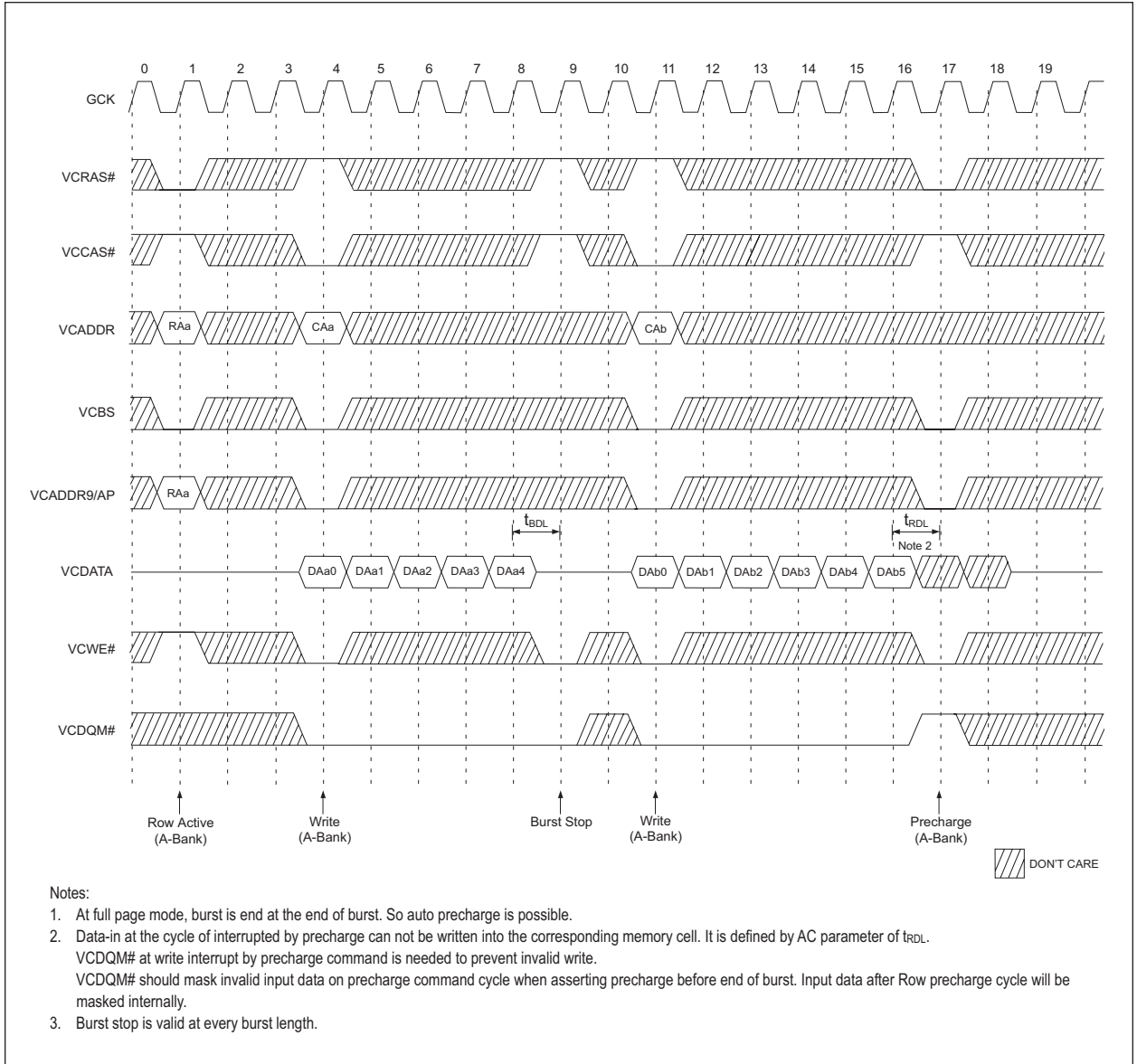
FIGURE 13 – SDRAM WRITE INTERRUPTED BY PRECHARGE COMMAND & WRITE BURST STOP @ BURST LENGTH = FULL PAGE
