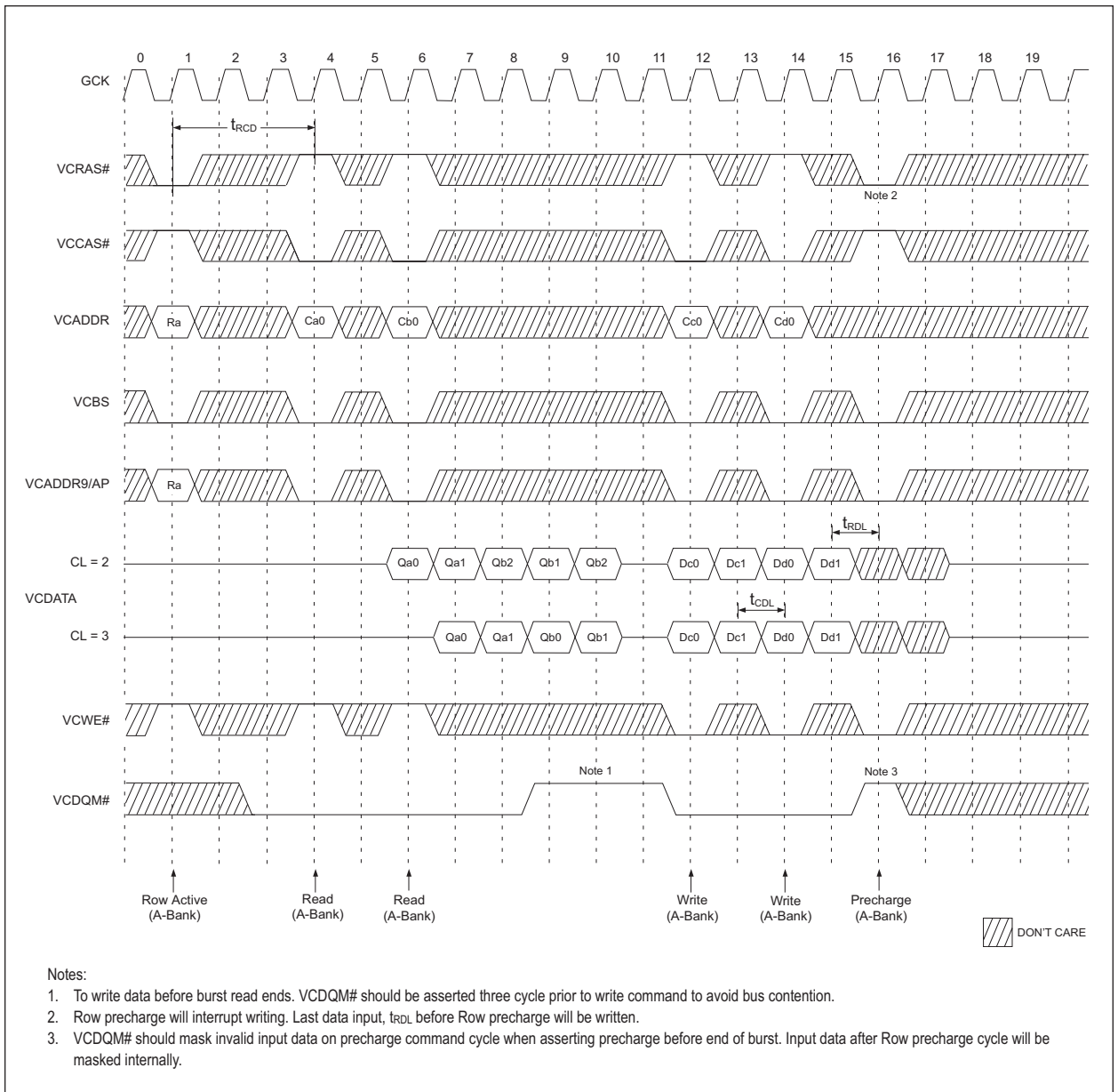
FIGURE 7 – SDRAM PAGE READ & WRITE CYCLE AT SAME BANK @ BURST LENGTH = 4
