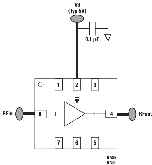
Figure 19. Typical Application.
