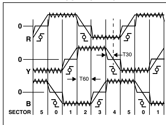
FIGURE 2: TYPICAL SENSORLESS COMMUTATION
