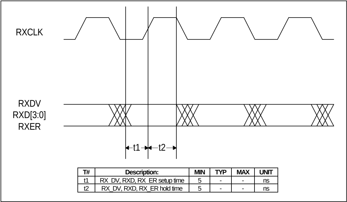
Figure-9.2a MII Receive Timing
