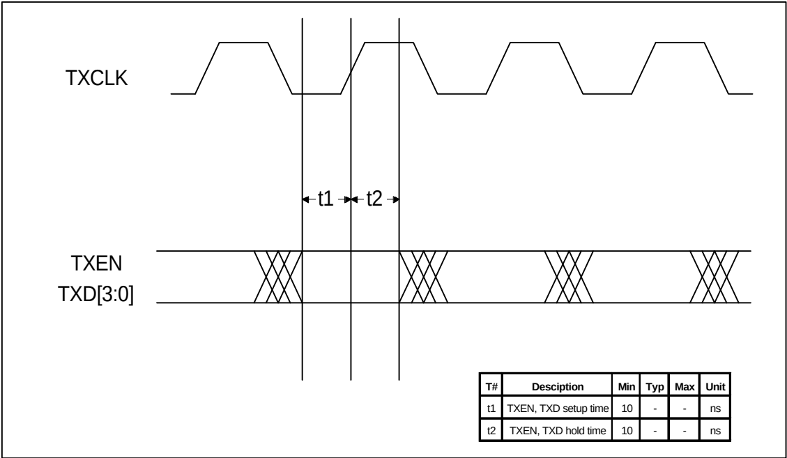
Figure-9.2b: MII Transmit Timing
