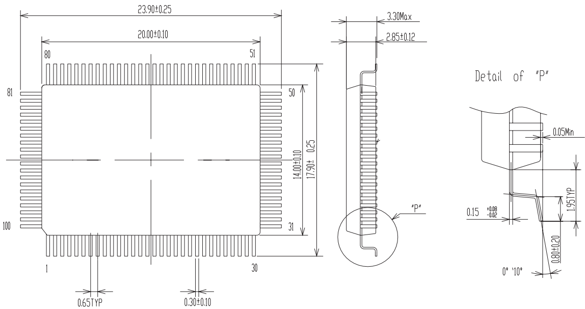
Figure 3: 100-pin EIAJ PQFP mechanical details
