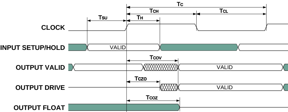
Figure 4: Clock and Synchronous Signals
