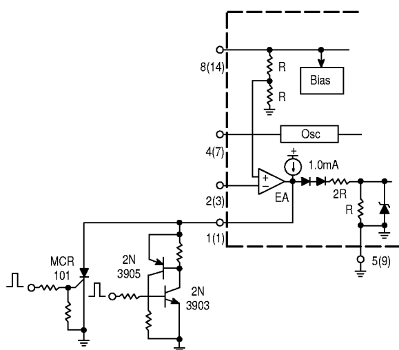
Figure 30. Latched Shutdown
