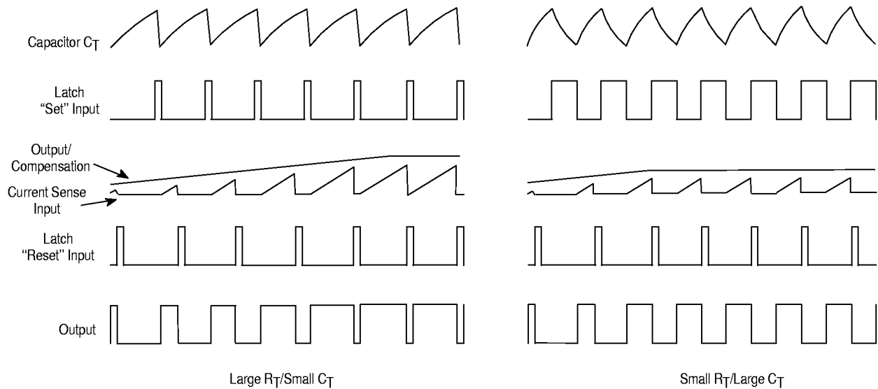
Figure 18. Timing Diagram
