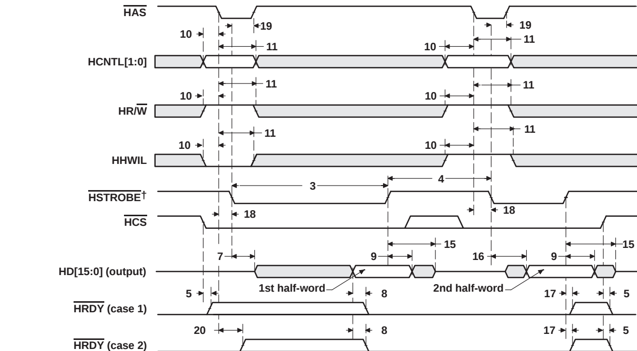
Figure 28. HPI Read Timing ( \overline{HAS} Used)
