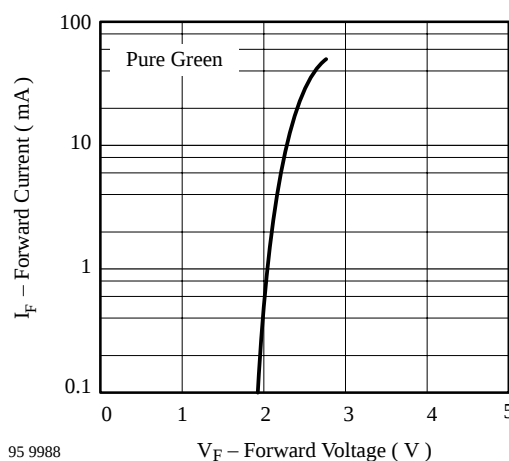
Figure 25 Forward Current vs. Forward Voltage
