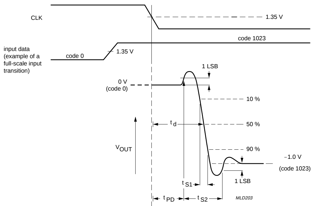
Fig.9 Switching characteristics.
