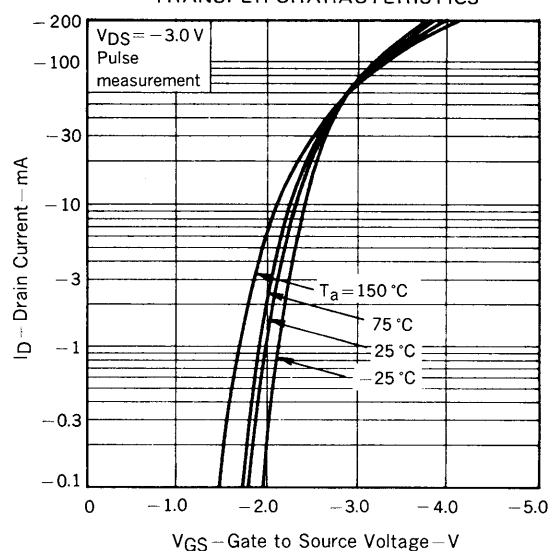
TRANSFER CHARACTERISTICS
