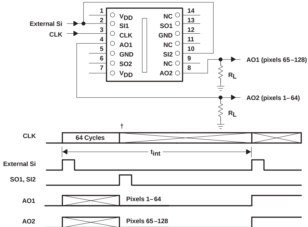
Figure 1. Serial Configuration
