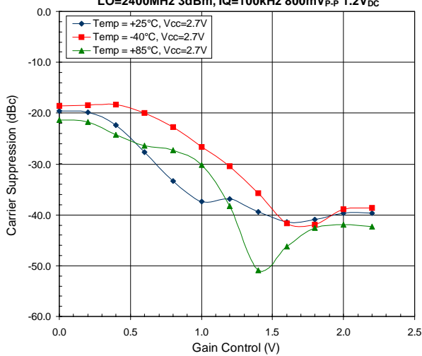
High Band Carrier Suppression versus Gain Control V_{CC}=2.7V , LO=2400MHz 3dBm , IQ=100kHz 800mV_{P-P} 1.2V_{DC}
