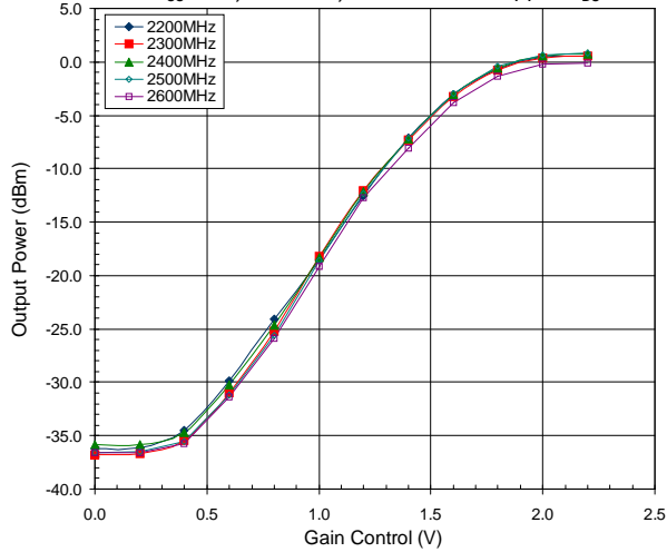
High Band Output Power versus Gain Control
