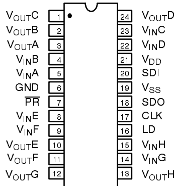
24 Pin PDIP (0.300")
