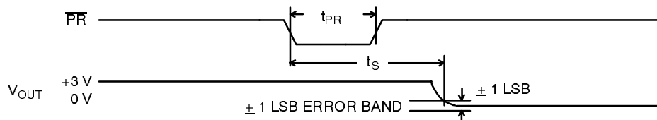
Figure 3. PRESET Operation
