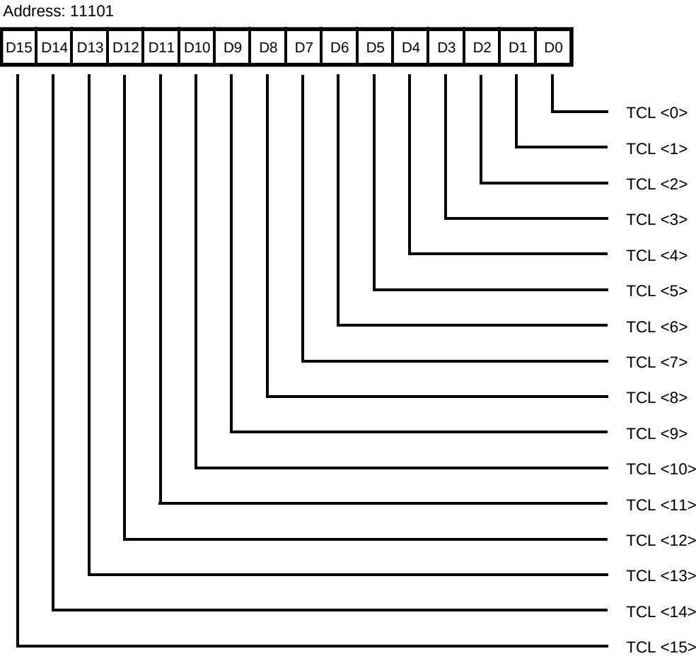
Figure 75. Transmit Count Limit Register (TCLR)
