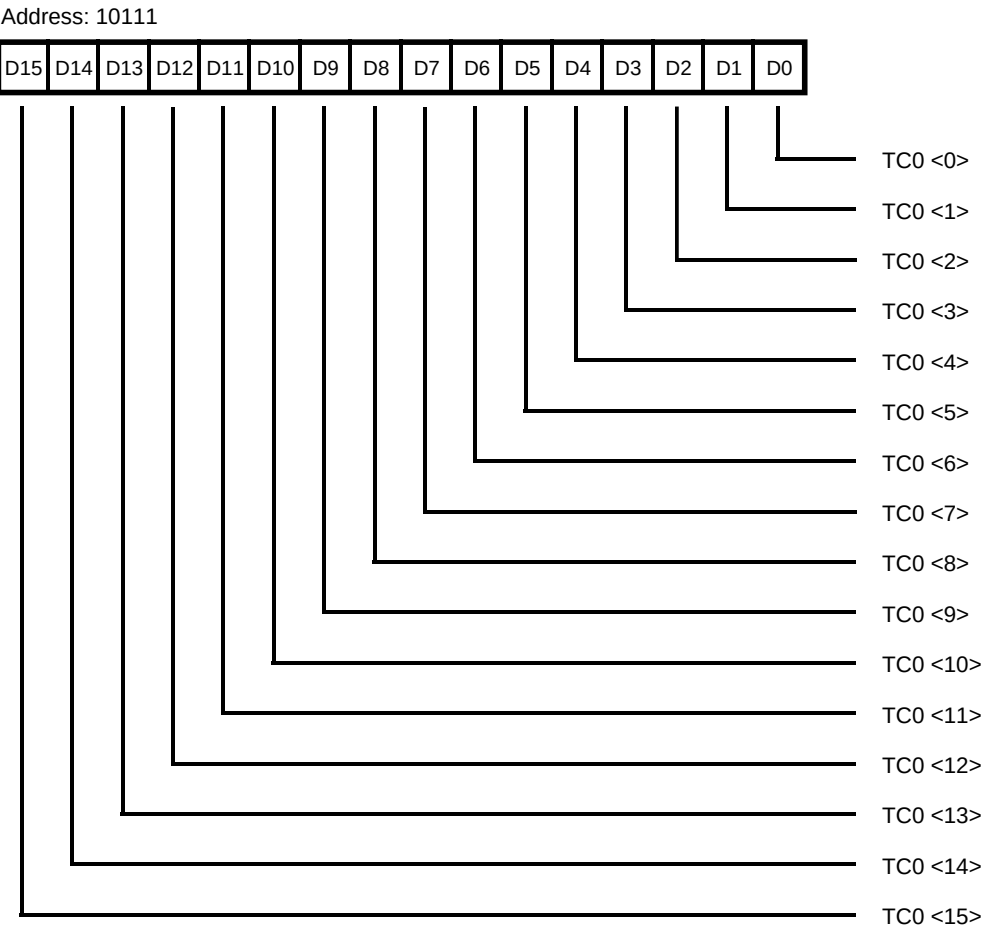
Figure 69. Time Constant 0 Register (TC0R)
