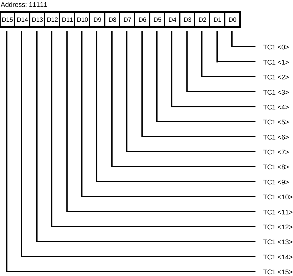
Figure 77. Time Constant 1 Register (TC1R)
