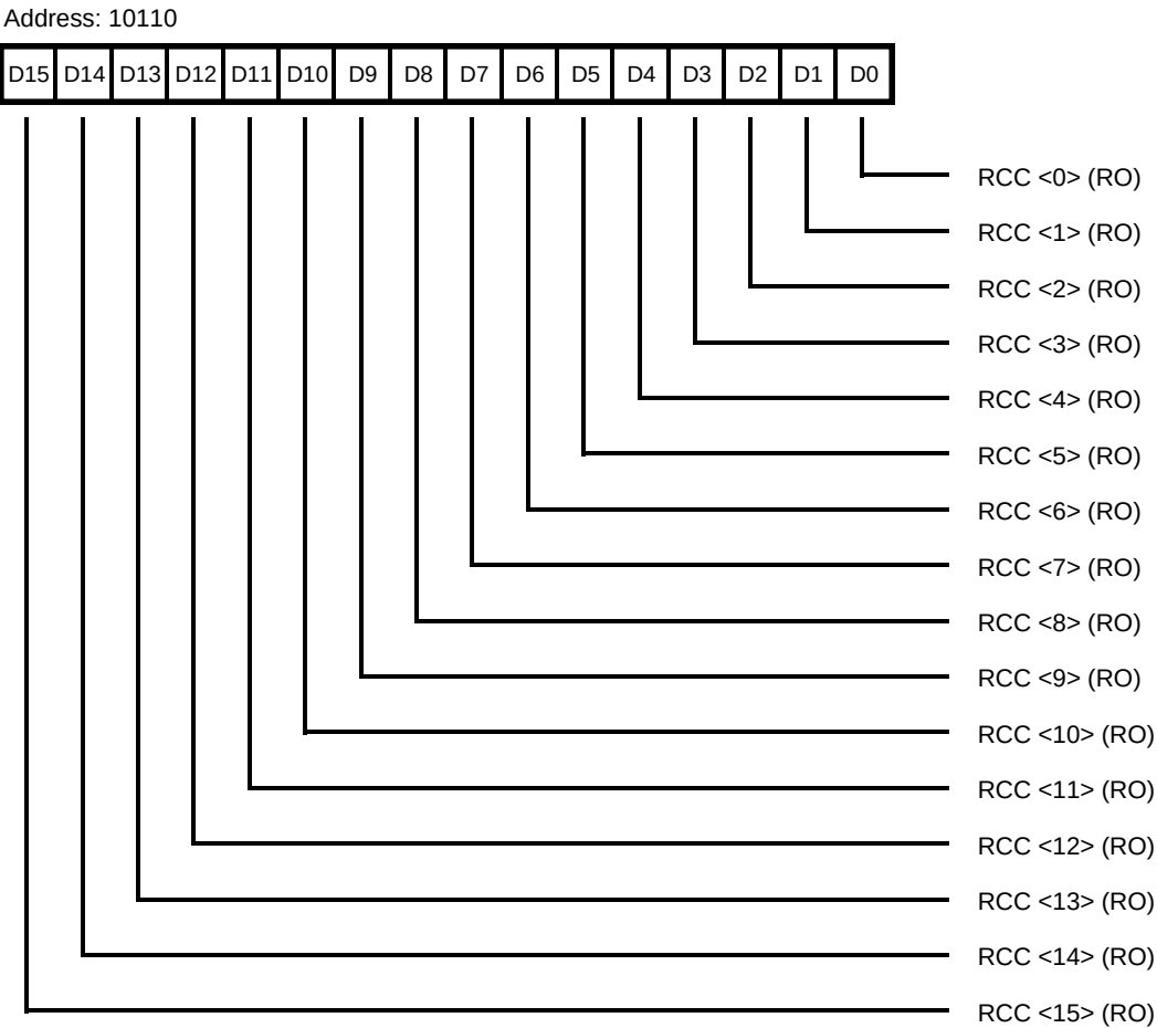
Figure 68. Receive Character Count Register (RCCR)
