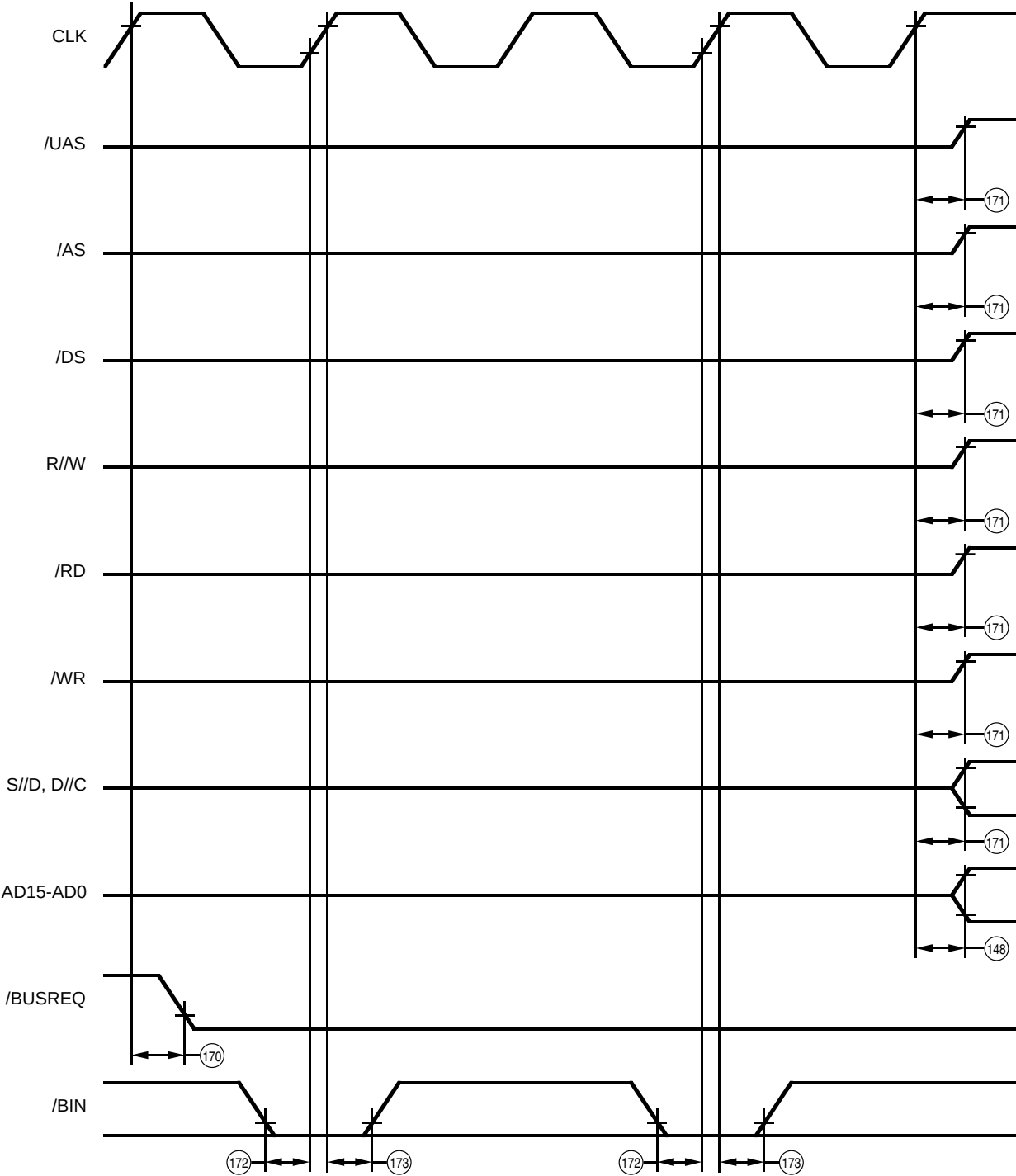
Figure 100. DMA Start-Up
