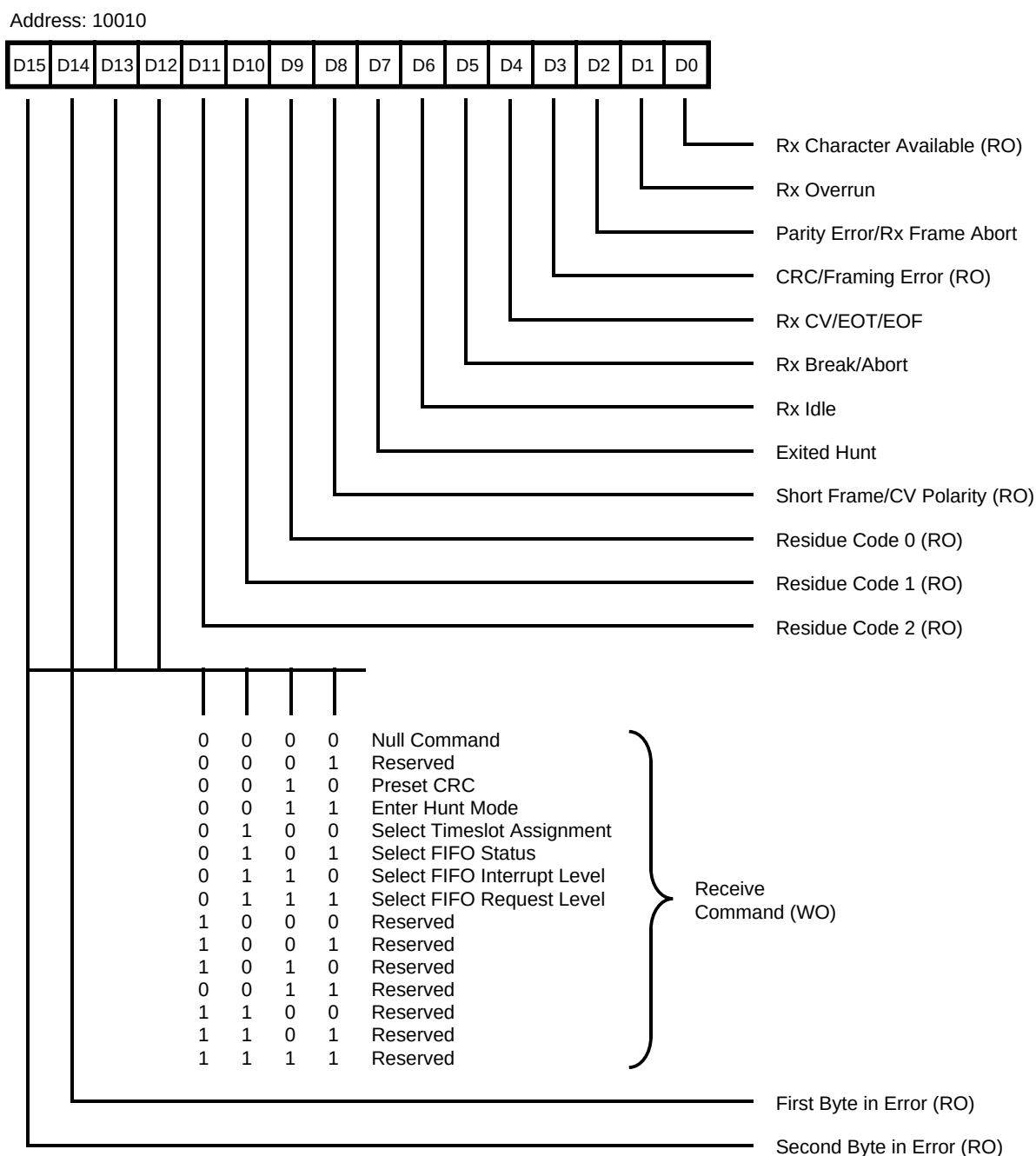
Figure 64. Receive Command Status Register (RCSR)
