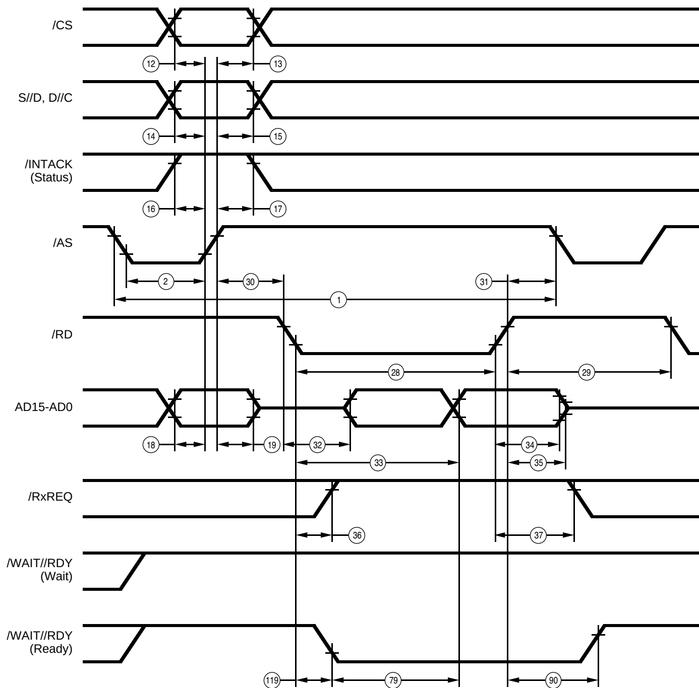
Figure 86. Multiplexed /RD Read Cycle
