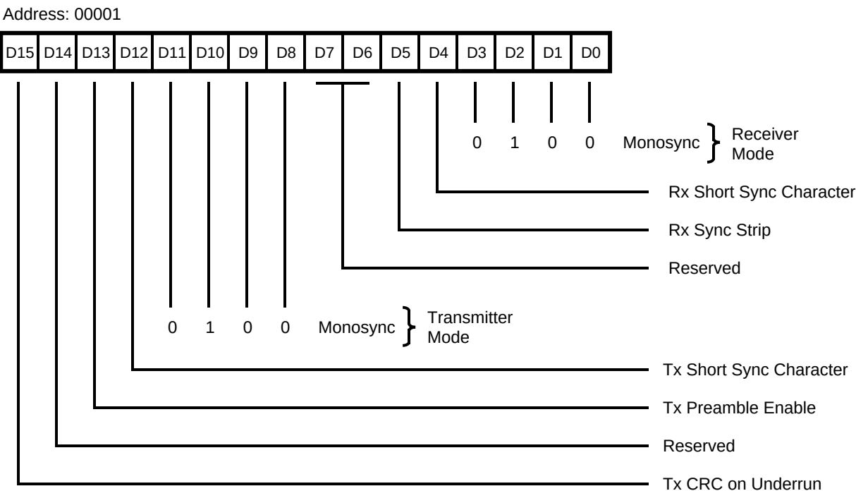
Figure 40. Channel Mode Register, Monosync Mode
