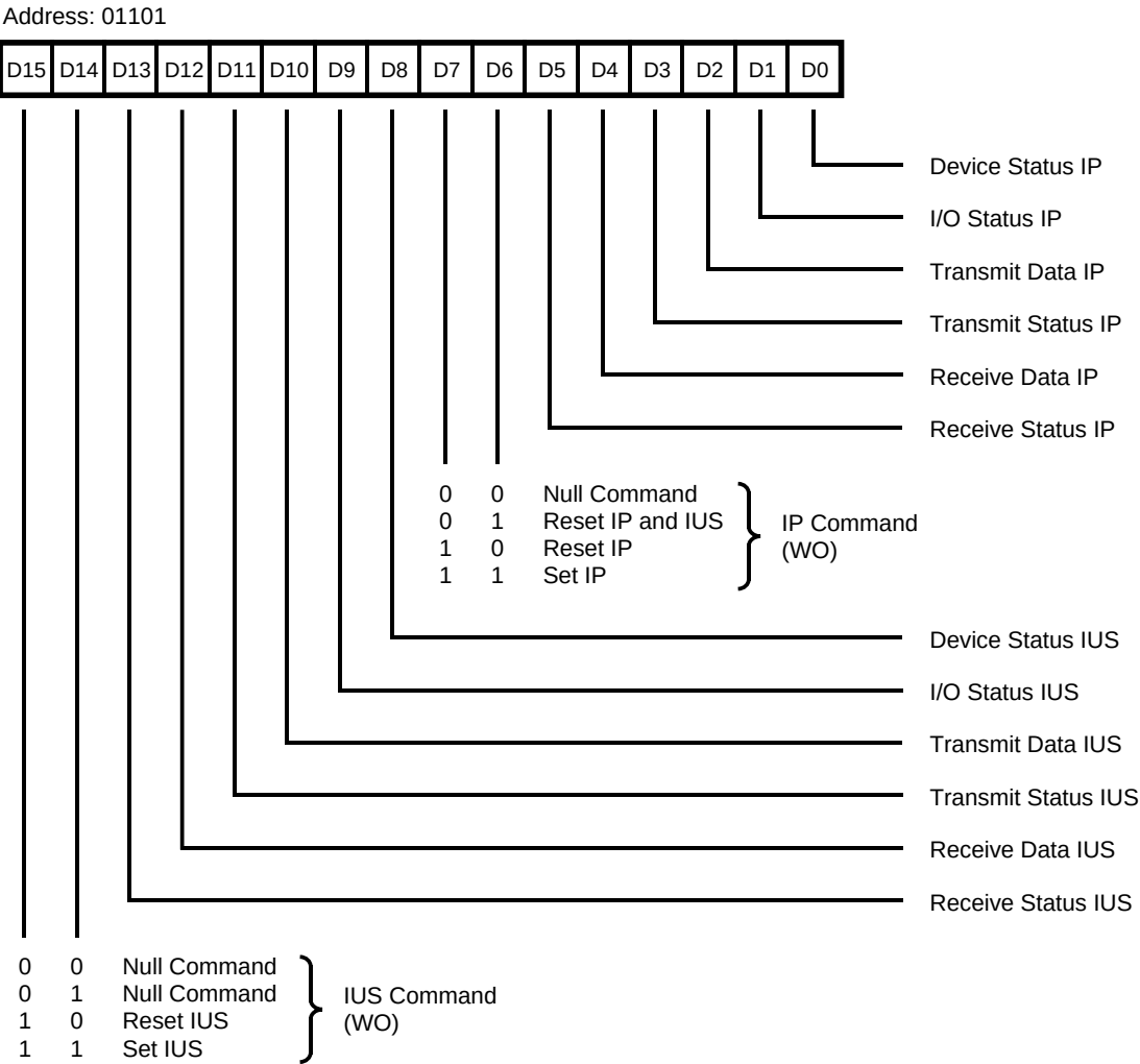
Figure 59. Daisy-Chain Control Register (DCCR)
