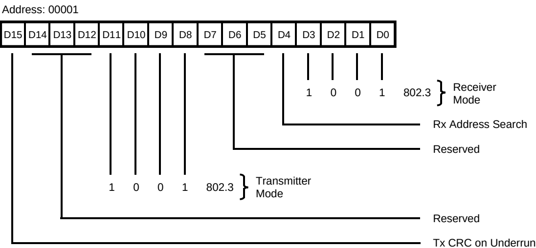
Figure 45. Channel Mode Register, 802.3 Mode
