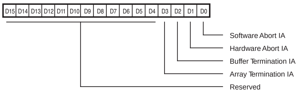
Figure 19. Tx/Rx DMA Interrupt Arm (TDIAR)/(RDIAR)
