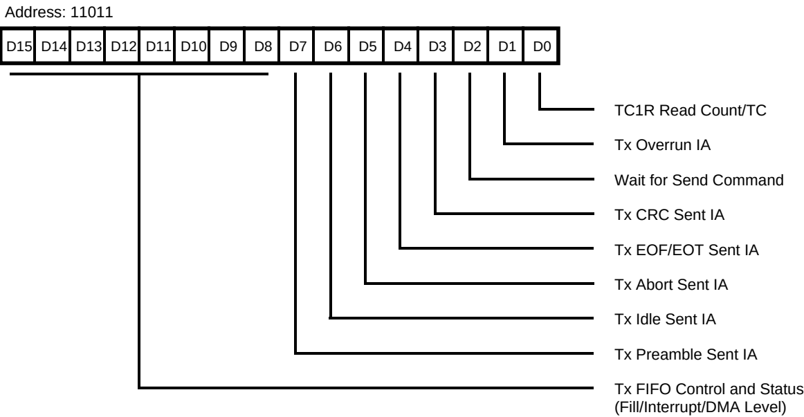
Figure 73a. Transmit Interrupt Control Register (TICR)
