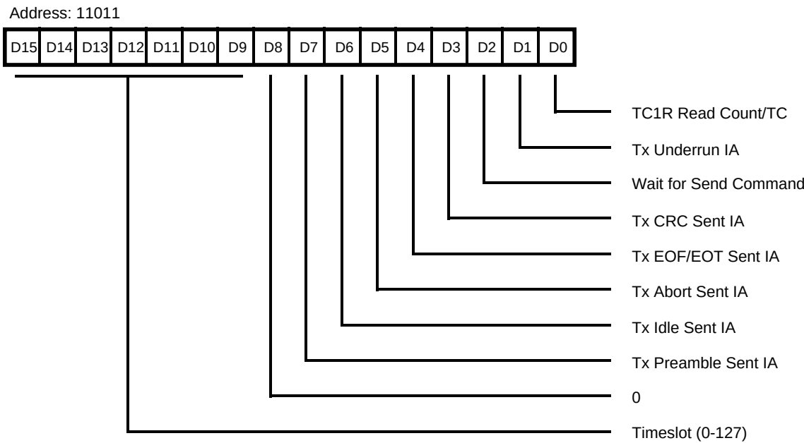
Figure 73b. Transmit Interrupt Control Register (TICR)
