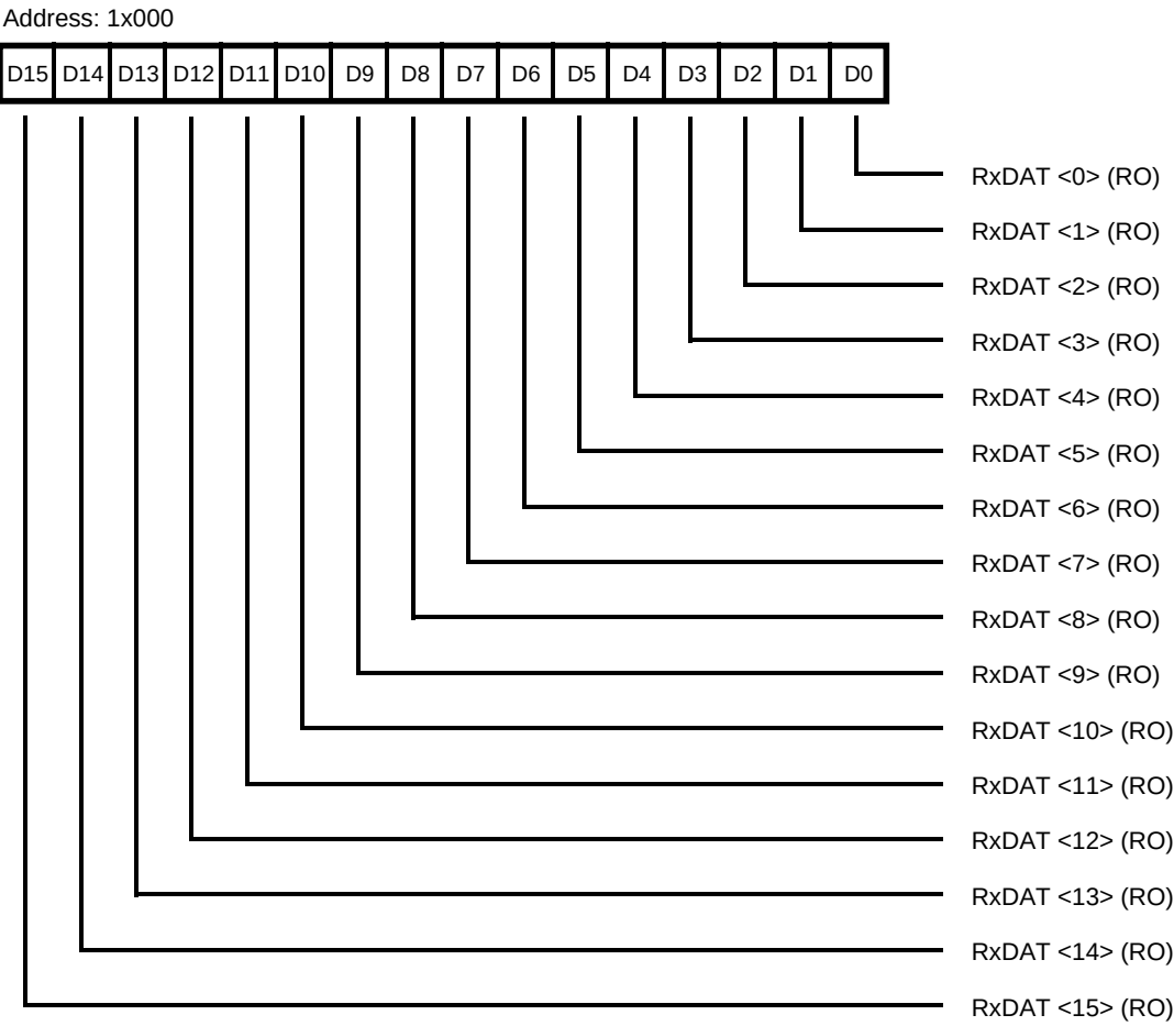
Figure 62. Receive Data Register (RDR)
