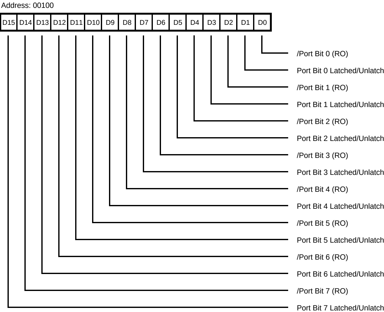
Figure 50. Port Status Register (PSR)
