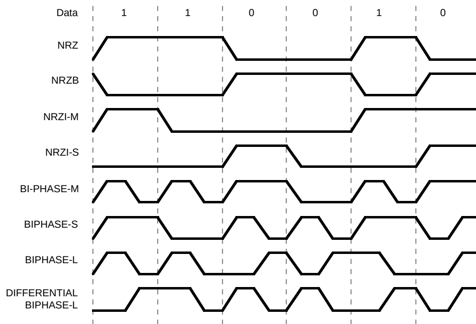
Figure 5. Data Encoding
