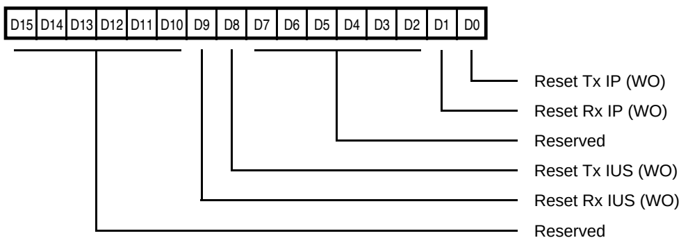
Figure 17. Clear DMA Interrupt Register (CDIR)
