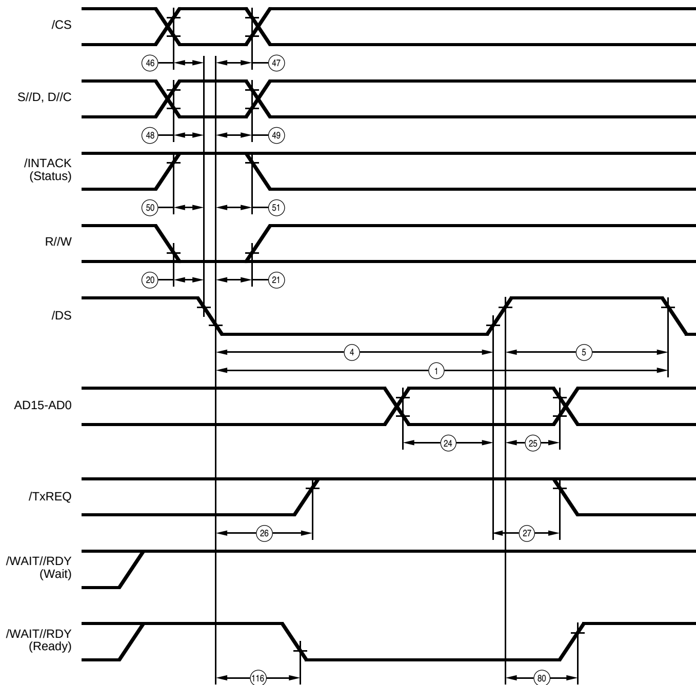
Figure 89. Non-Multiplexed /DS Write Cycle
