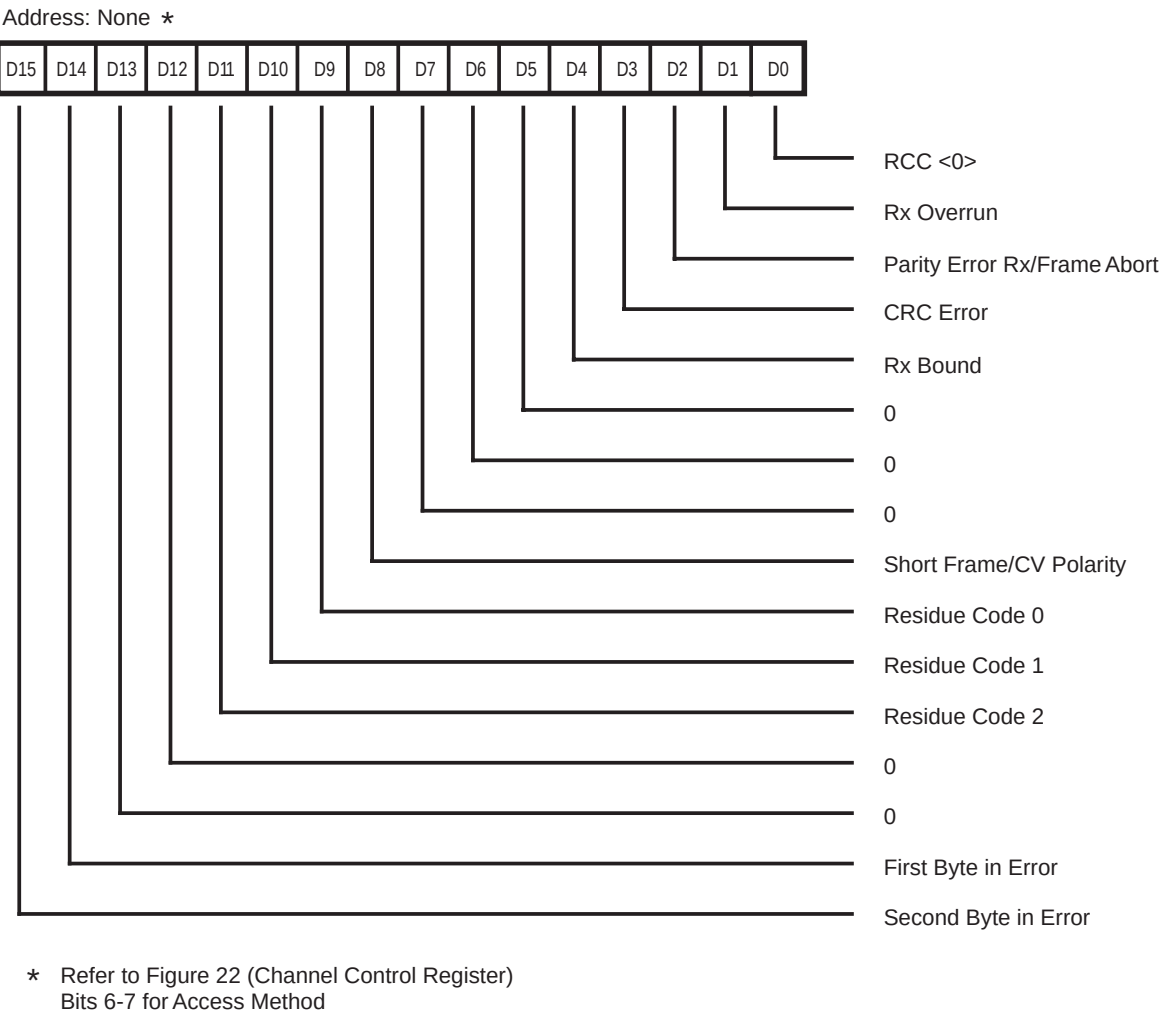
Figure 78. Receive Status Block Register (RSBR)
