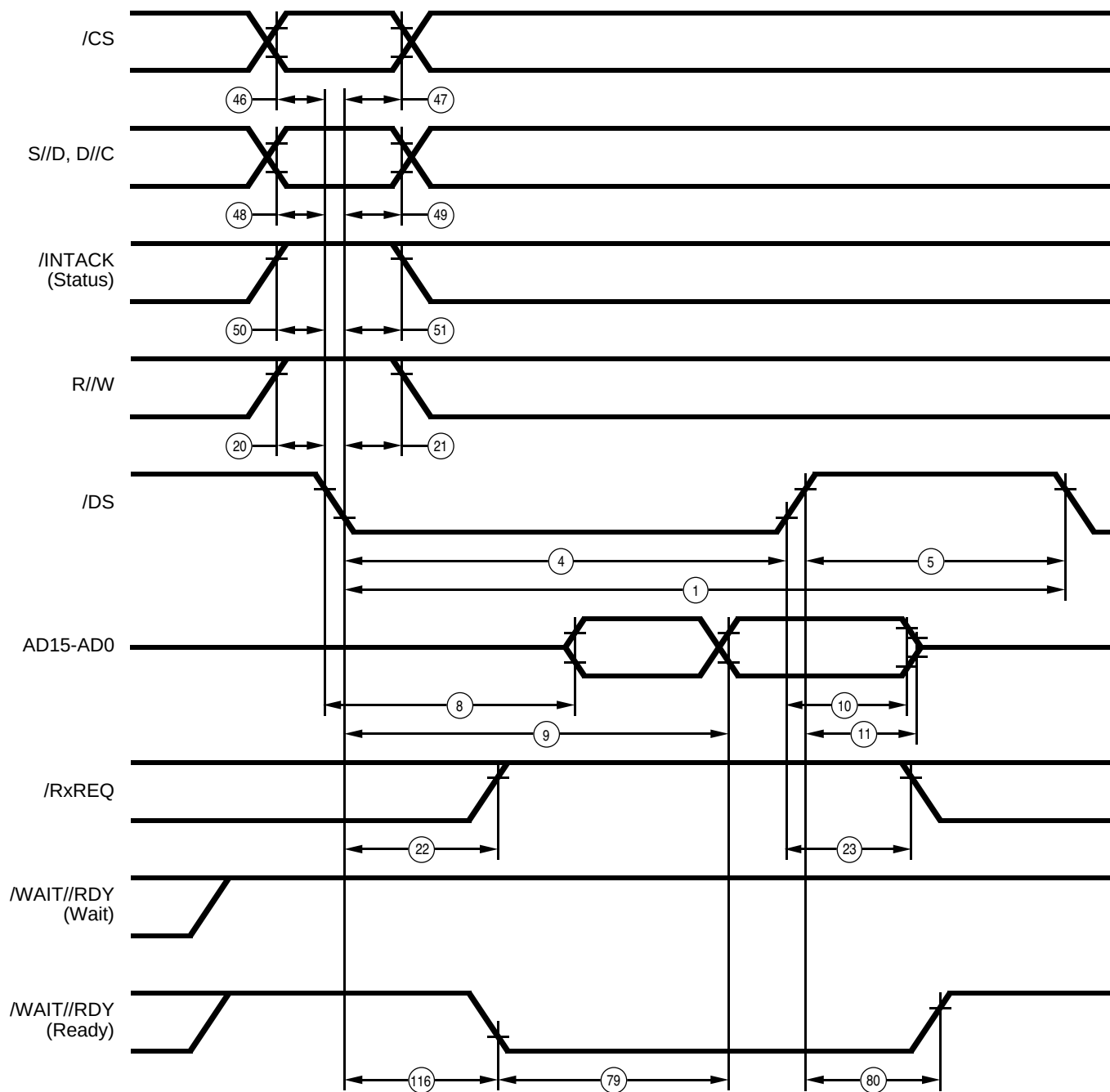
Figure 88. Non-Multiplexed /DS Read Cycle
