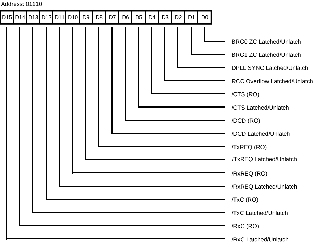
Figure 60. Miscellaneous Interrupt Status Register (MISR)
