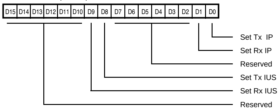
Figure 18. Set DMA Interrupt Register (SDIR)
