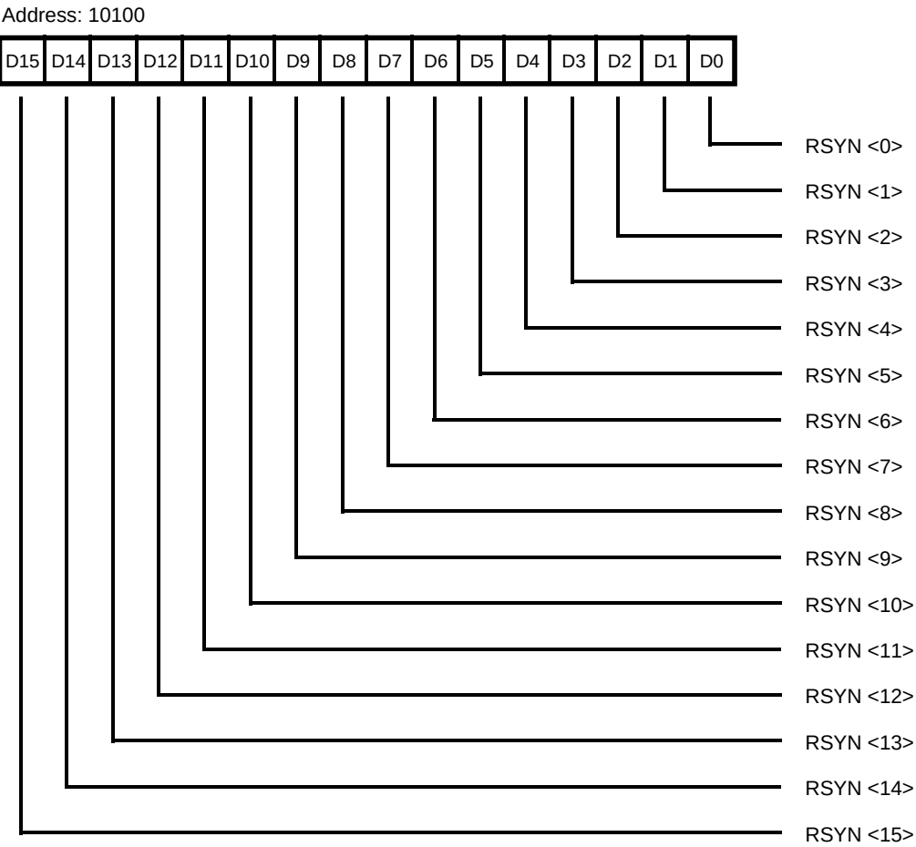
Figure 66. Receive Sync Register (RSR)
