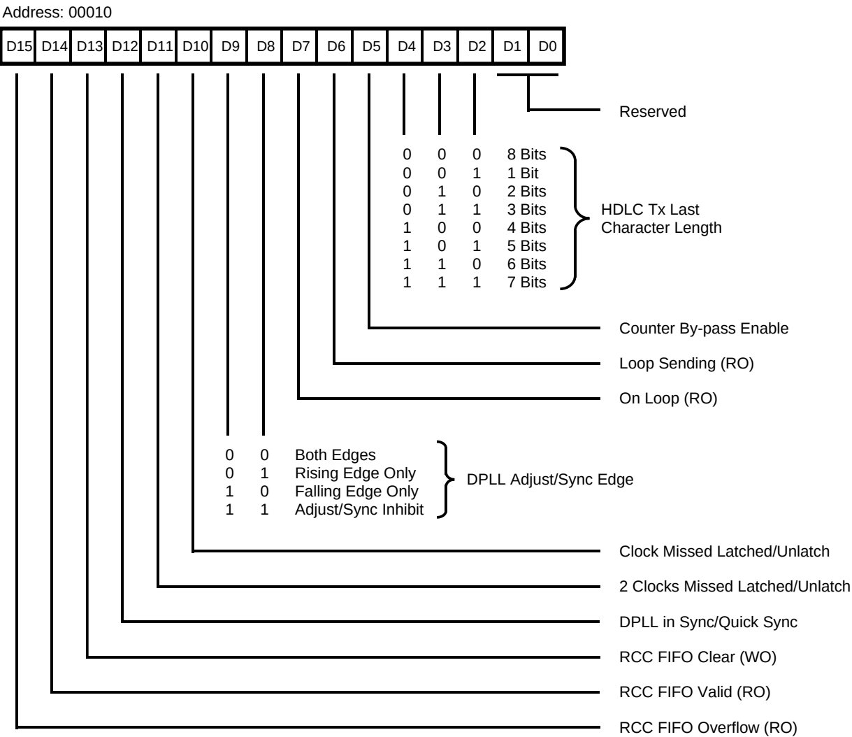
Figure 48. Channel Command/Status Register (CCSR)
