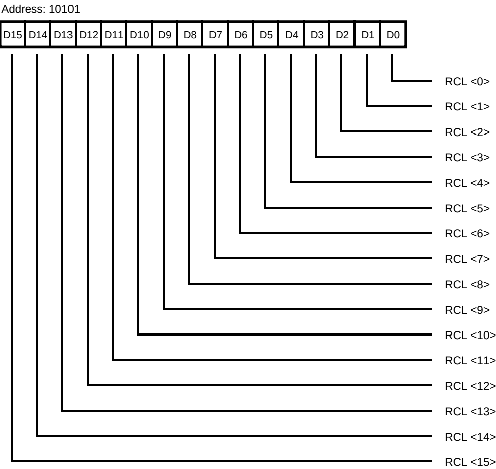
Figure 67. Receive Count Limit Register (RCLR)
