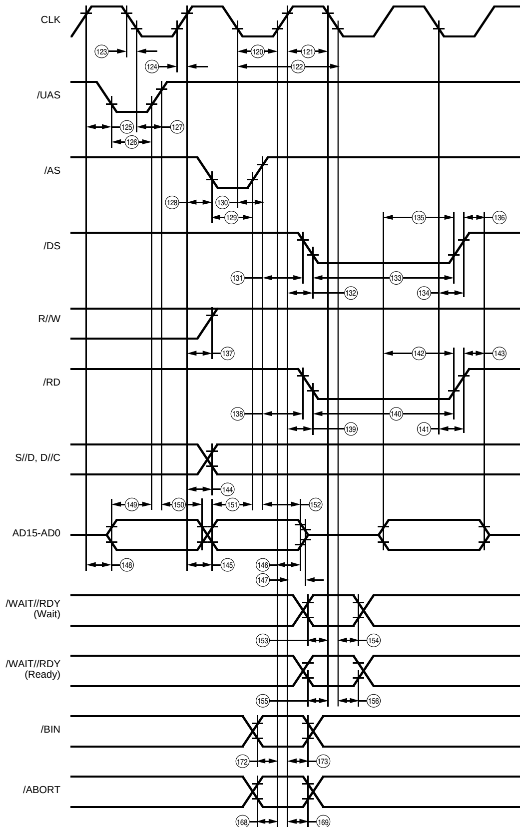
Figure 101. Memory Read
