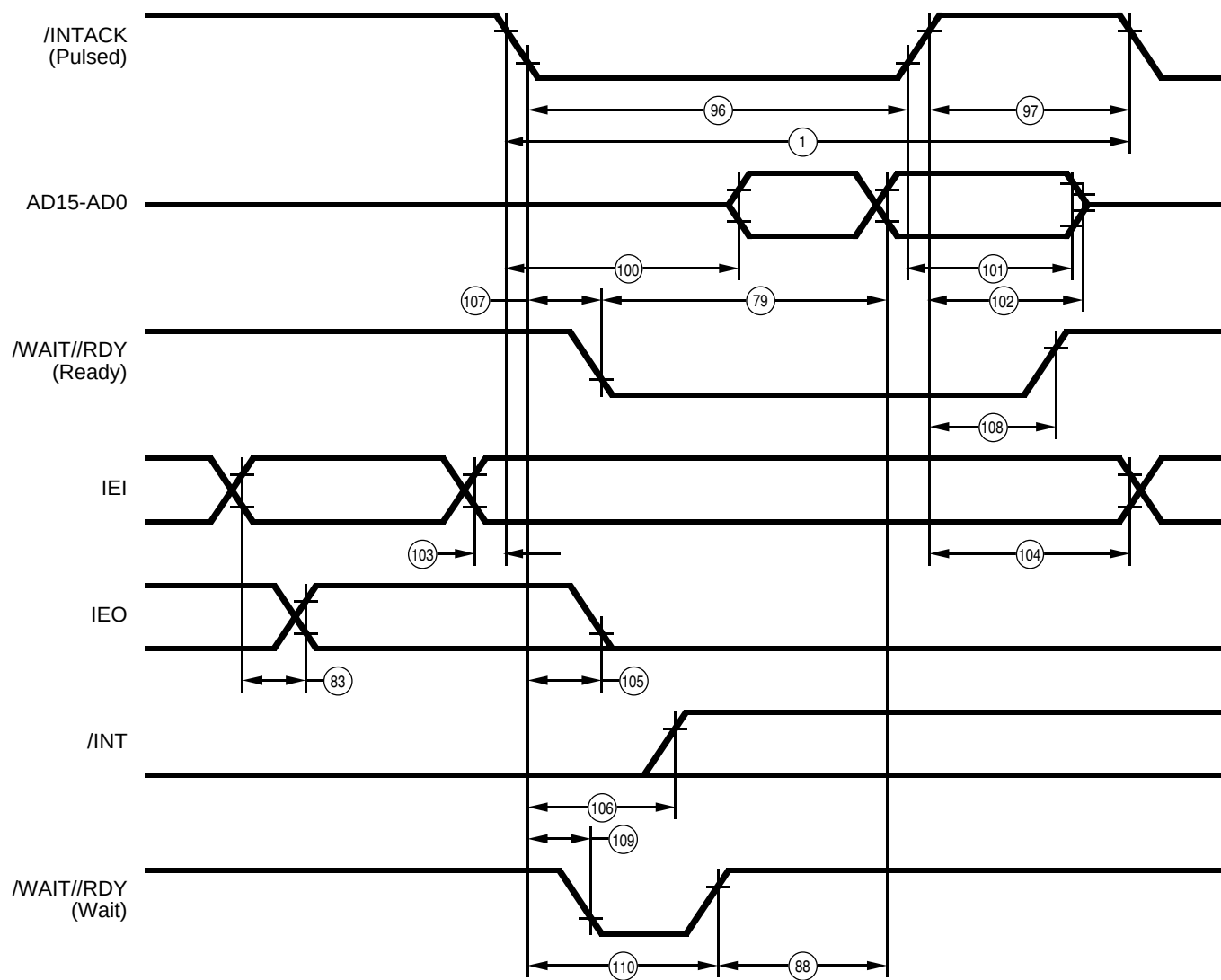
Figure 97. Non-Multiplexed Pulsed Interrupt Acknowledge Cycle
