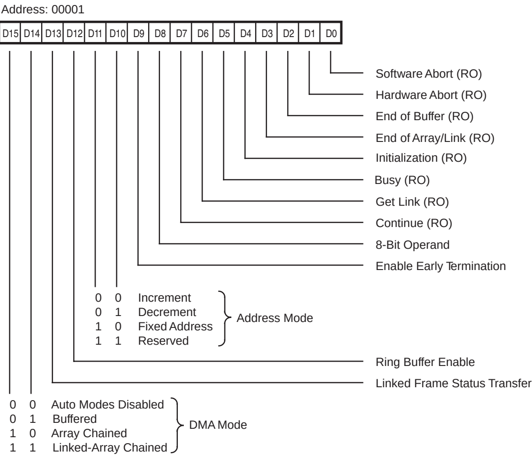
Figure 9. Tx/Rx DMA Mode Register (TDMR) (RDMR)
