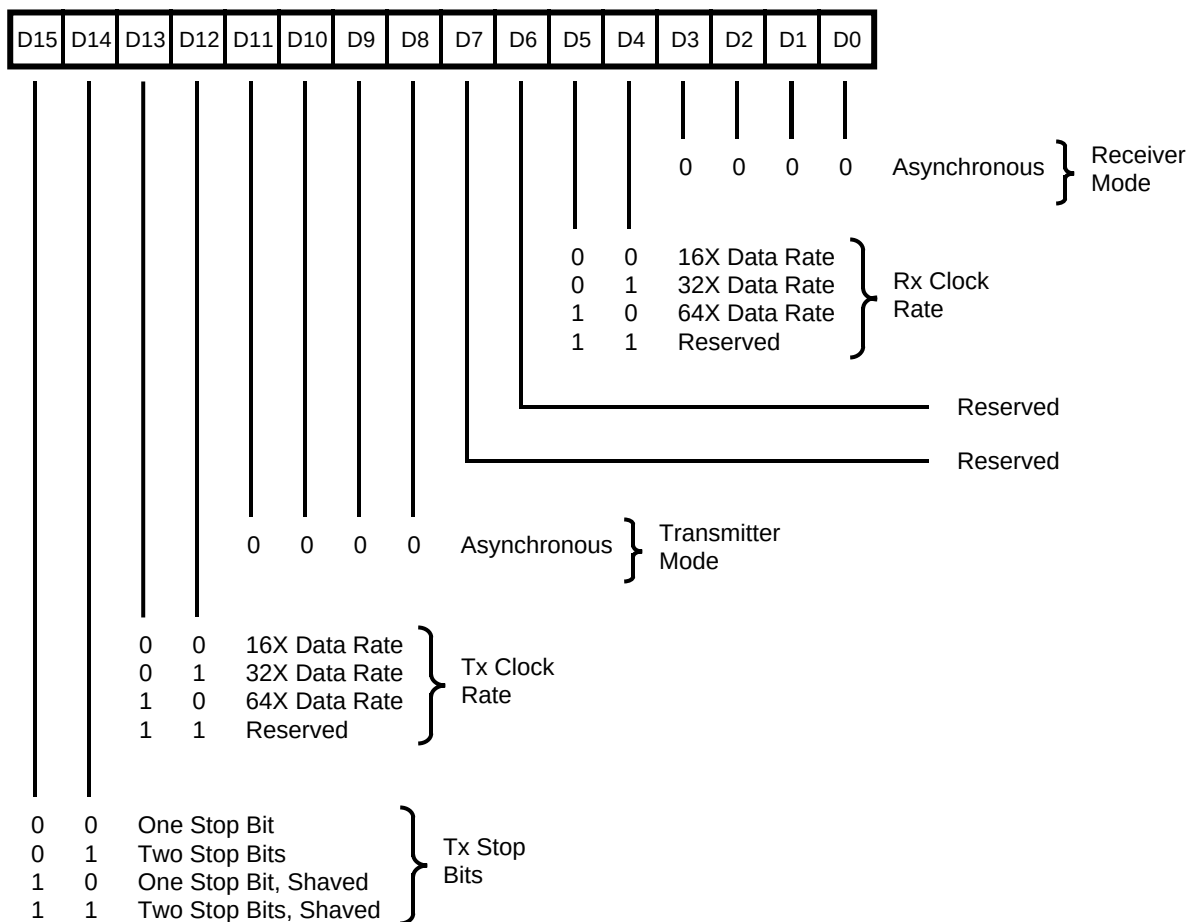
Figure 36. Channel Mode Register, Asynchronous Mode
