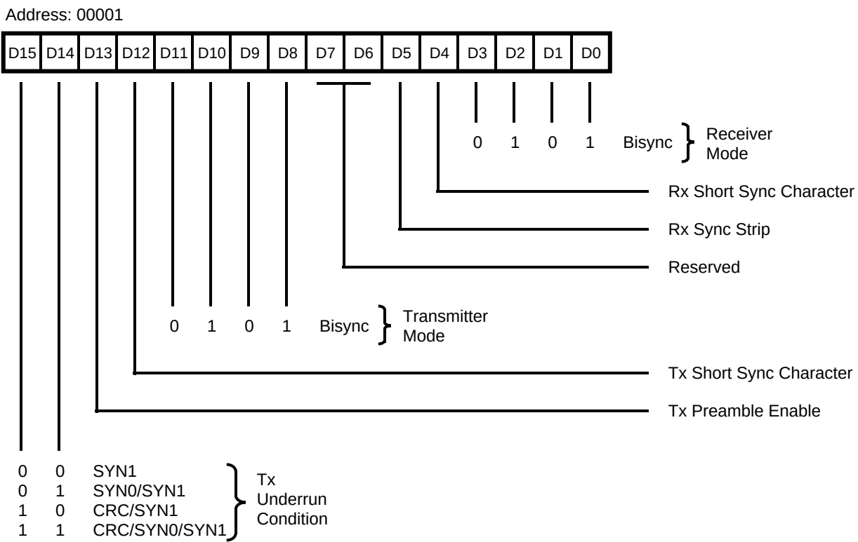
Figure 41. Channel Mode Register, Bisync Mode
