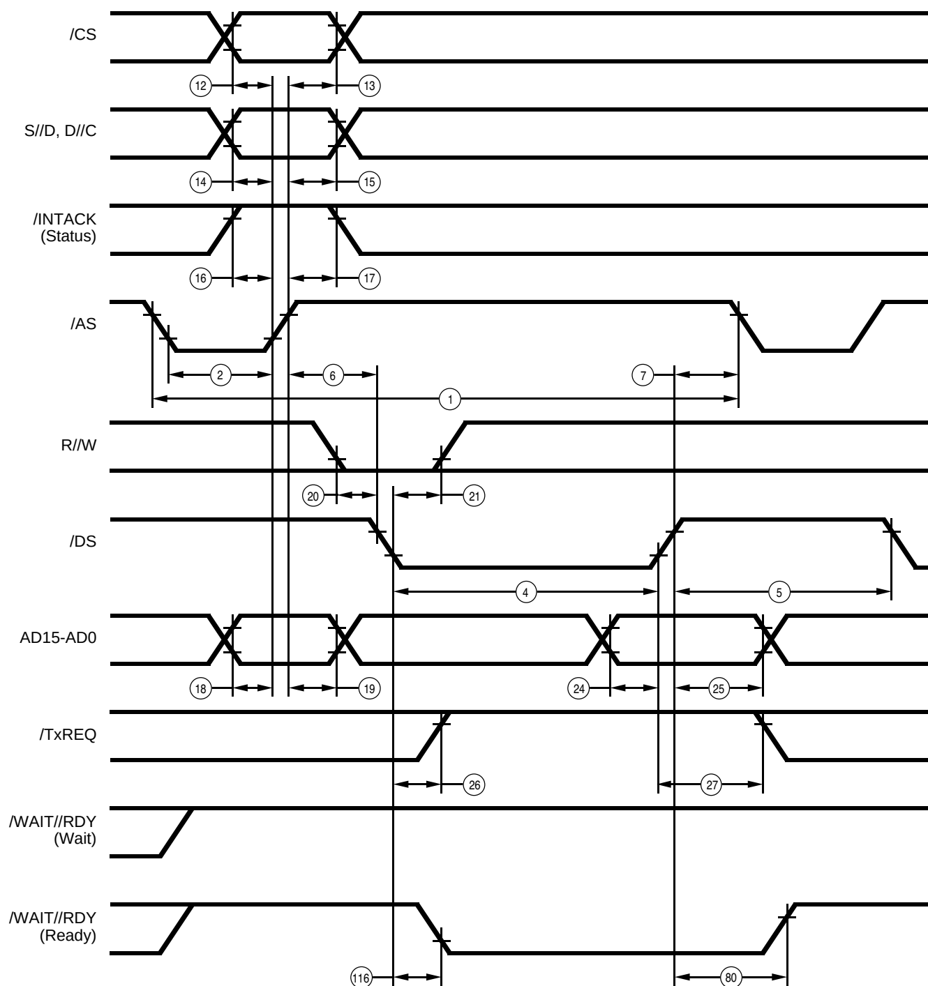
Figure 85. Multiplexed /DS Write Cycle
