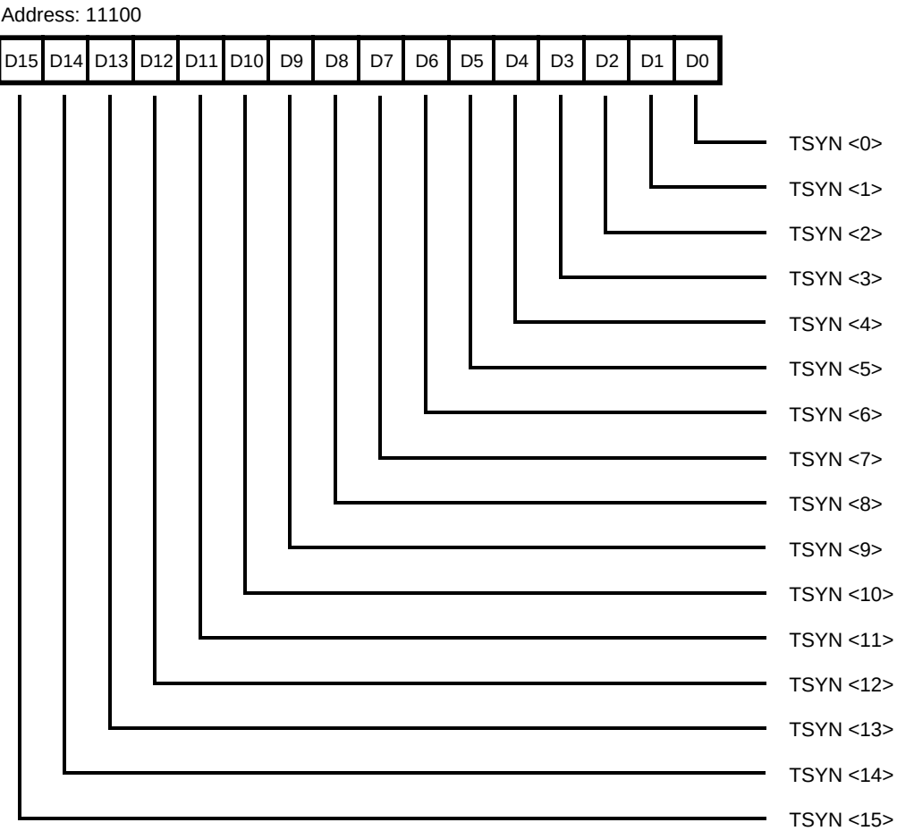
Figure 74. Transmit Sync Register (TSR)
