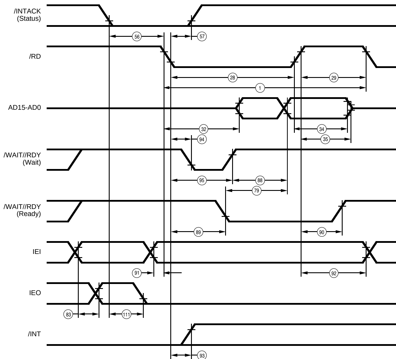
Figure 96. Non-Multiplexed /RD Pulsed Interrupt Acknowledge Cycle
