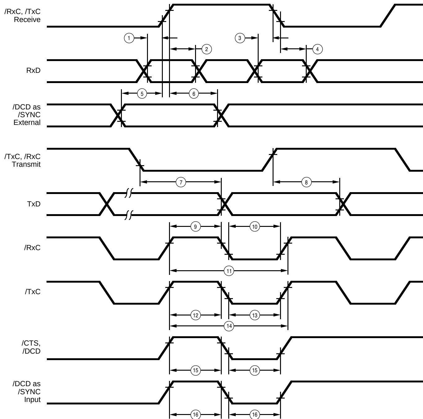
Figure 105. General Timing
