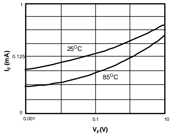
Forward Characteristic
