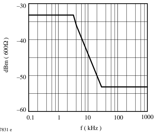
Figure 2 DTMF distortion
