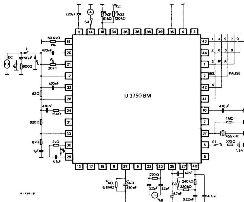
Figure 3 Test circuit
