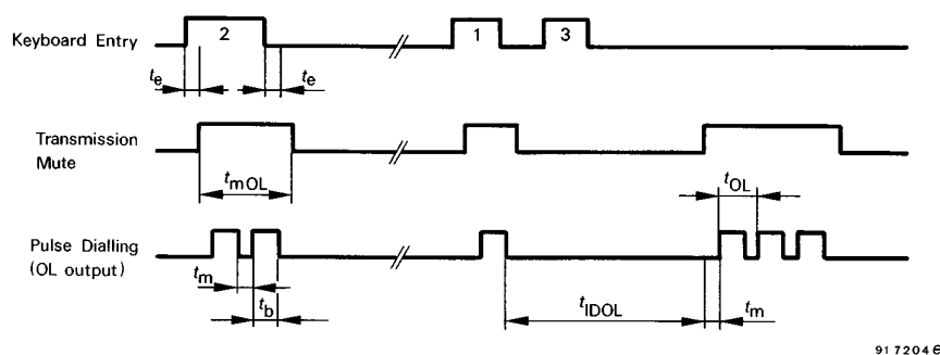
Figure 12 Timing diagram for pulse dialing
