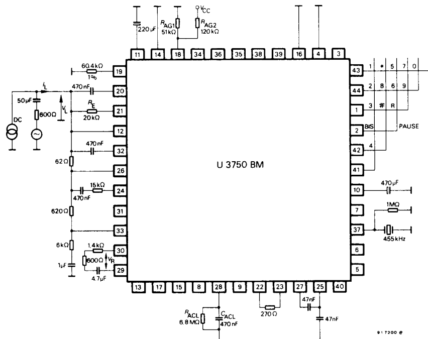
Figure 4 Test circuit
