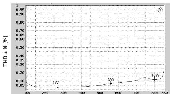
Output Power
