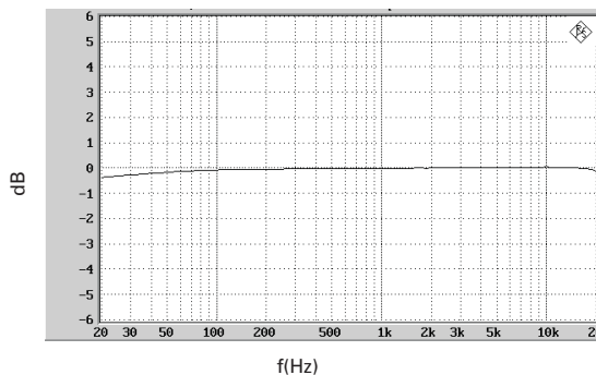
Frequency response (8Ω load)
