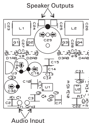
Figure 7. Class D 25W Mono O.L. PCB Silk Screen (Actual Size)
