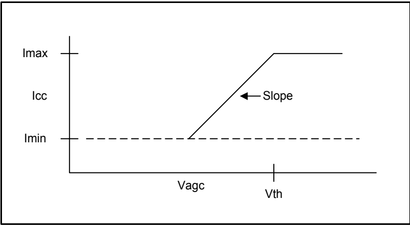
Figure 13 - Transmit Output Stage Current versus Gain Control
