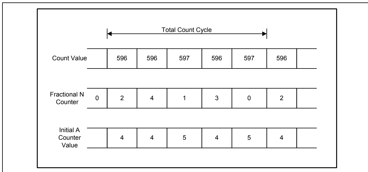
Figure 10 - UHF Synthesizer - Fractional N Operation
