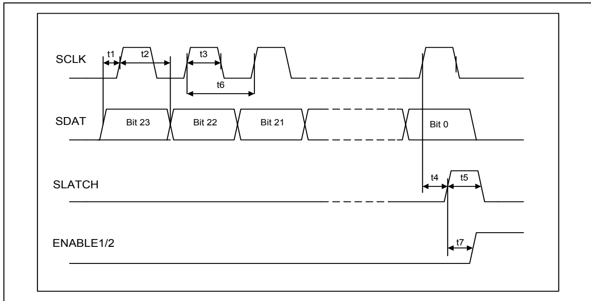
Figure 12 - Serial Bus Timing
