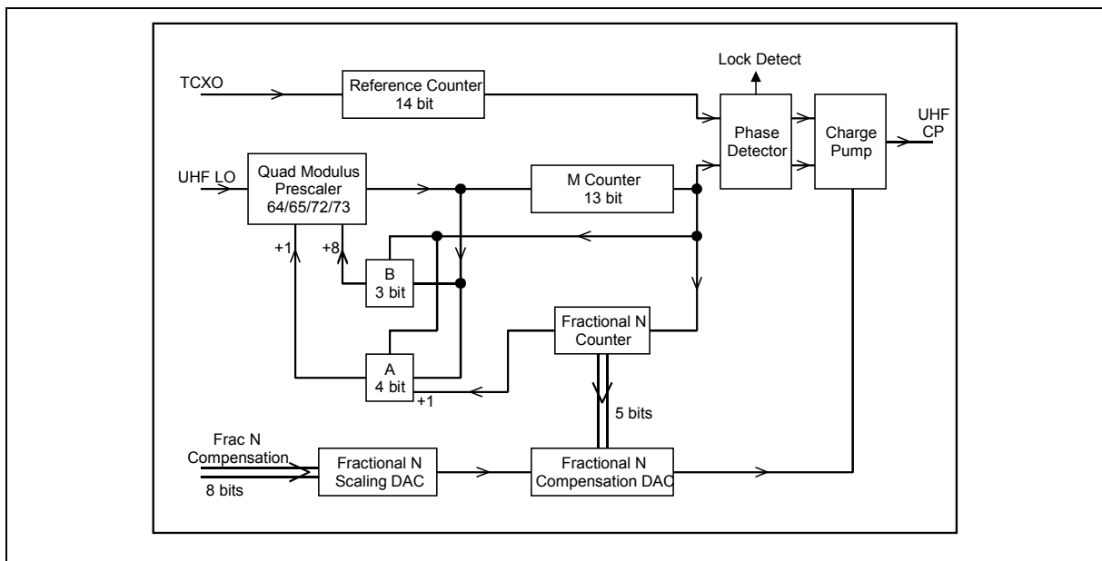
Figure 8 - UHF Synthesizer
