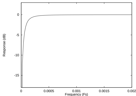
Figure 22 ADC Highpass Filter Response
