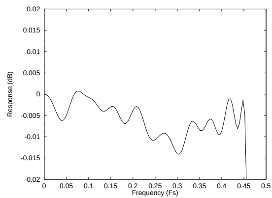
Figure 21 ADC Digital Filter Ripple
