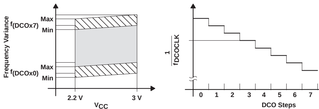
Figure 13. DCO Characteristics
