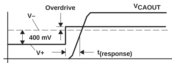
Figure 10. Overdrive Definition
