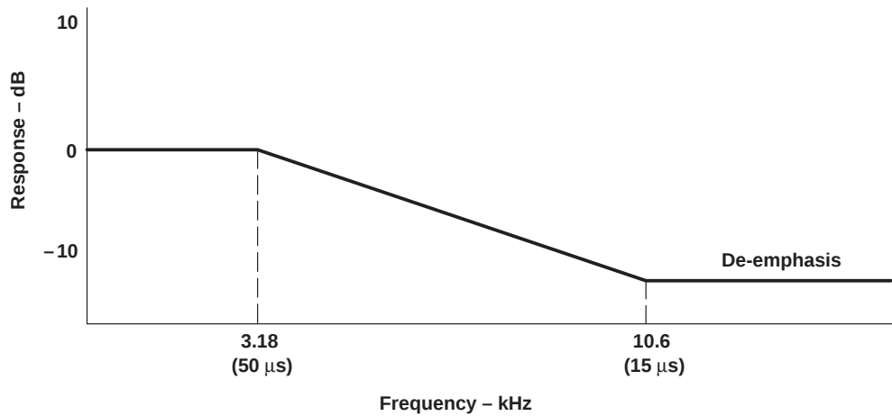
Figure 4. De-emphasis Characteristics
