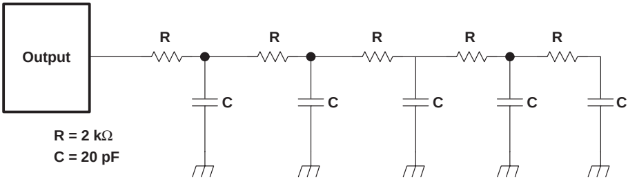
Figure 7. Load Circuit
