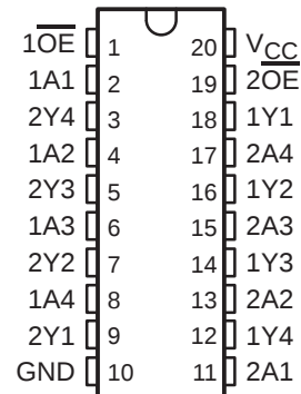
SN54ABT240 . . . J PACKAGE SN74ABT240 . . . DB, DW, OR N PACKAGE (TOP VIEW)
