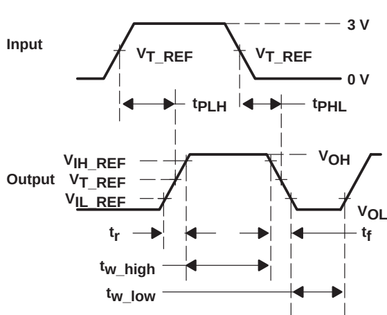
VOLTAGE WAVEFORMS
