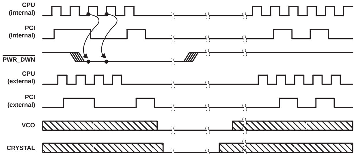
Figure 5. Power-Down Timing
