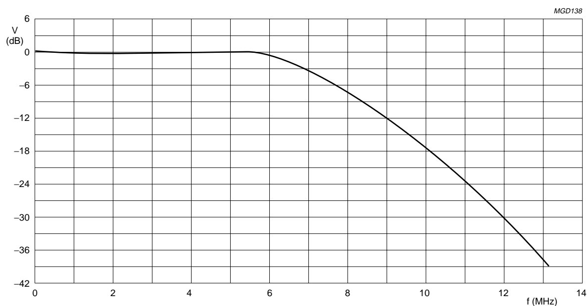
Fig.3 Anti-alias filter.
