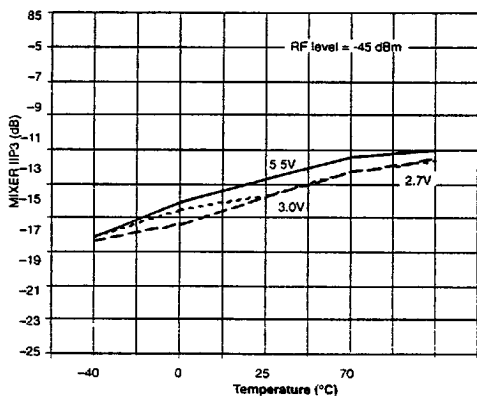
Mixer IIP3 at 240MHz vs Temperature and Supply Voltage
