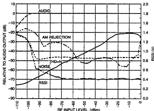
Receiver RF Performance — T = -40^{\circ}\text{C} , Audio Level = 118\text{mV}_{\text{RMS}}
