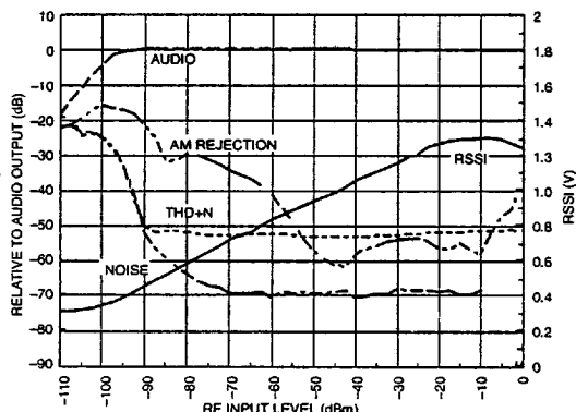
Receiver RF Performance — T = 25^{\circ}\text{C} , Audio Level = 129\text{mV}_{\text{RMS}}
