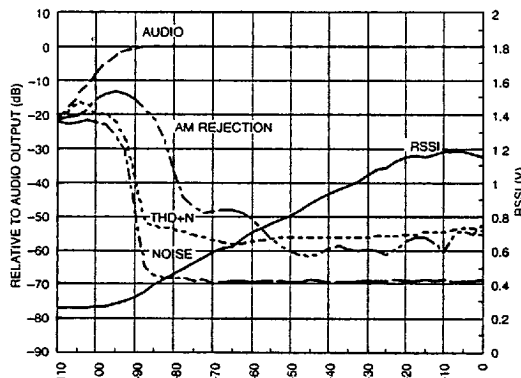
Receiver RF Performance — T = 85^{\circ}\text{C} , Audio Level = 131\text{mV}_{\text{RMS}}
