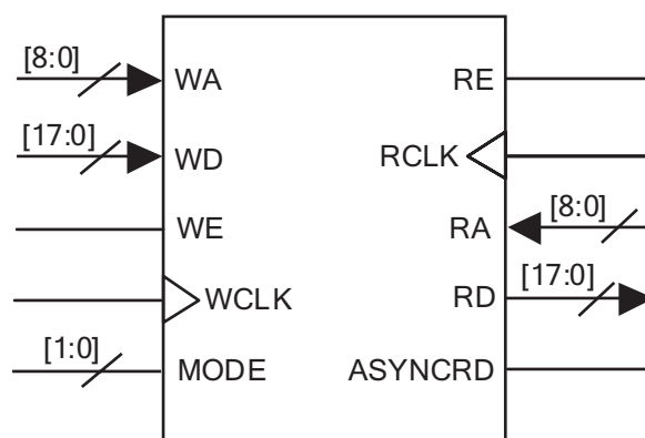
Figure 2: QuickRAM Module
