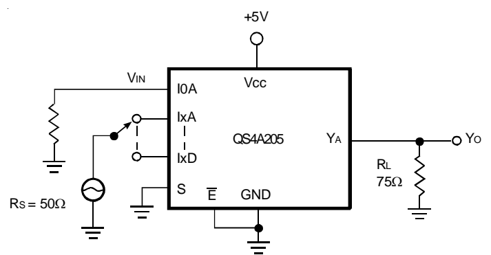
Crosstalk
