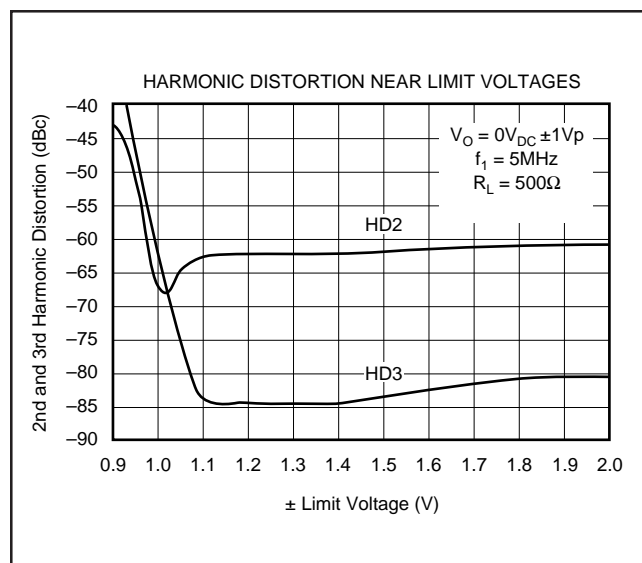
FIGURE 8. Linearity Guardband.
