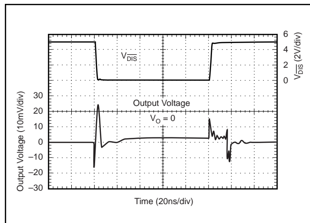
FIGURE 18. Disable/Enable Glitch.
