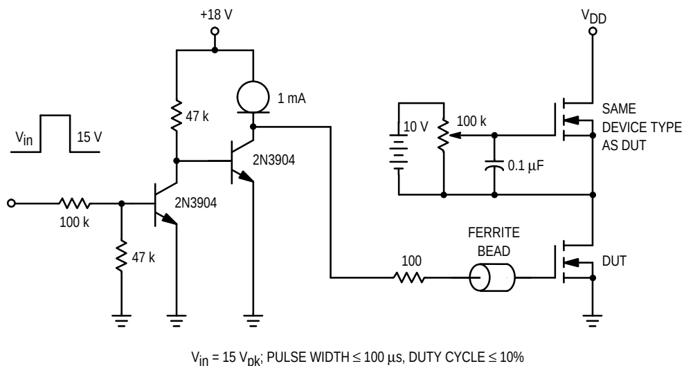
Figure 20. Gate Charge Test Circuit
