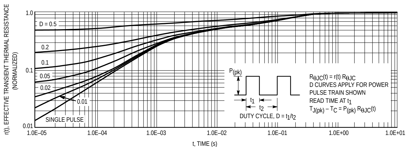
Figure 13. Thermal Response
