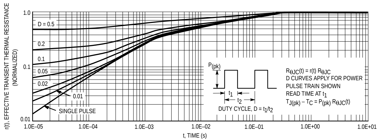
Figure 14. Thermal Response
