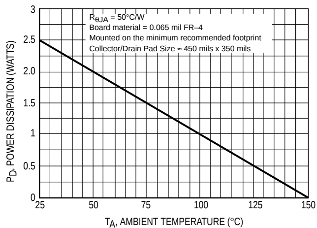
Figure 16. D 2 PAK Power Derating Curve
