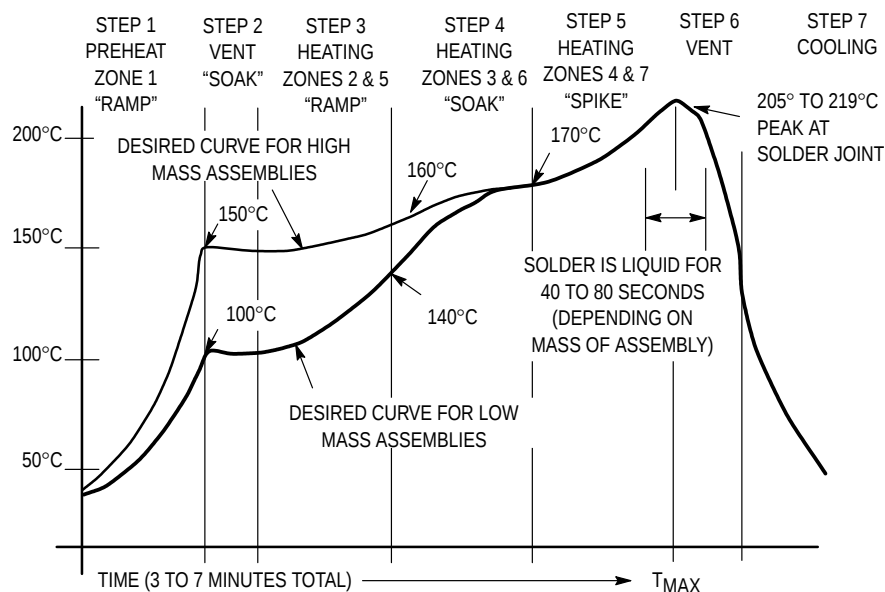
Figure 19. Typical Solder Heating Profile
