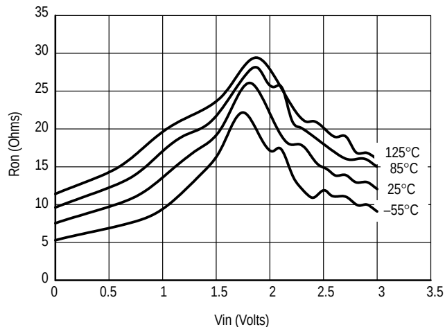
Figure 1c. Typical On Resistance, V_{CC} = 3.0\text{ V}
