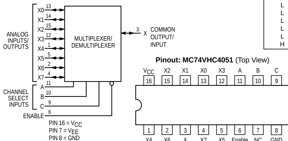
LOGIC DIAGRAM MC74VHC4051 Single-Pole, 8-Position Plus Common Off
