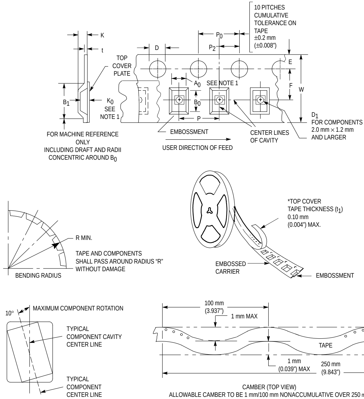
Figure 5. Carrier Tape Specifications
