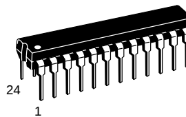
N SUFFIX PLASTIC CASE 724-03
