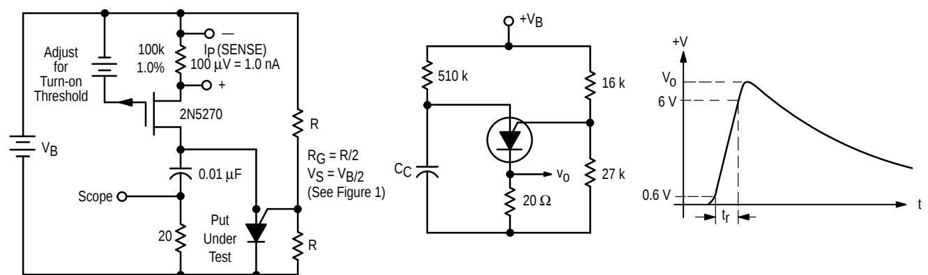
FIGURE 2 – PEAK CURRENT ( I_P ) TEST CIRCUIT
