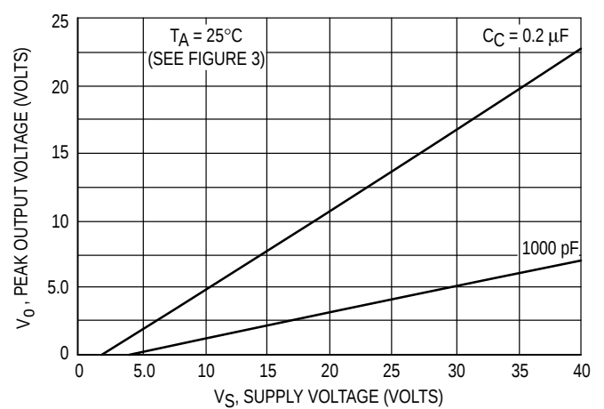
FIGURE 7 – PEAK OUTPUT VOLTAGE
