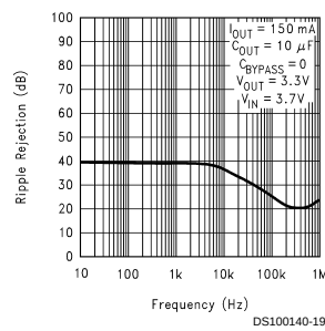
Ripple Rejection
