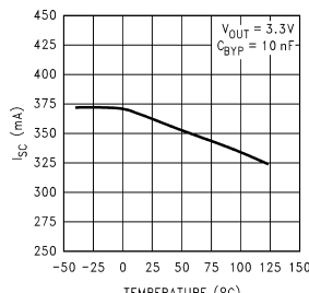
Instantaneous Short Circuit Current
