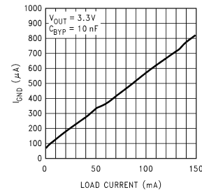
Ground Pin vs Load Current
