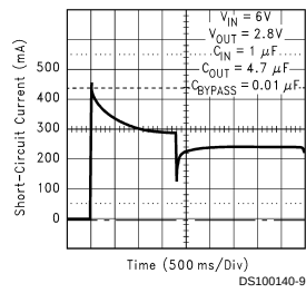
Short-Circuit Current
