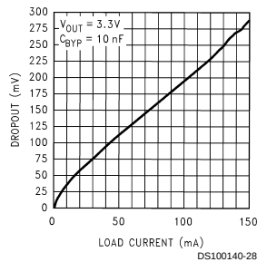
Dropout Voltage vs Load Current
