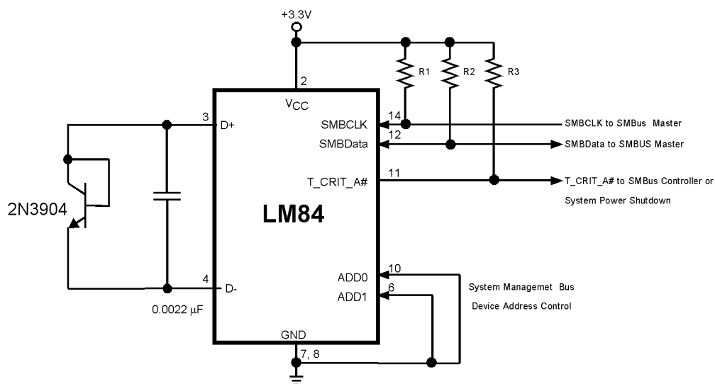
Using a Diode Connected 2N3904 as a Remote Temperature Sensing Element
