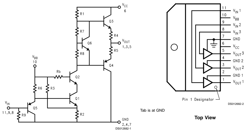
FIGURE 1. Simplified Schematic Diagram (One Channel)
