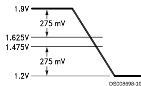
FIGURE 9. Noise Margin
