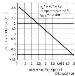
Zero Error Change vs Reference Voltage
