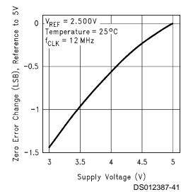
Zero Error Change vs Supply Voltage
