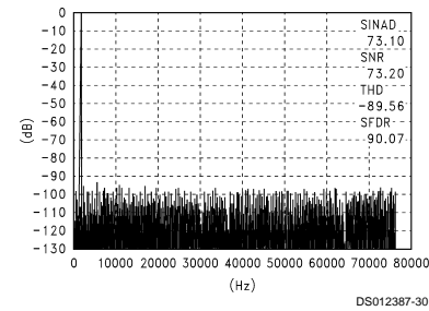
Half Scale Differential 1 kHz Sine Wave Input, f_s = 153.6 kHz
