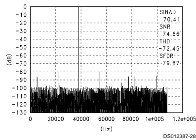
Full Scale Differential 38,452 Hz Sine Wave Input
