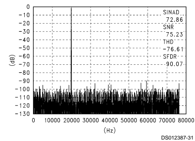
Half Scale Differential 20 kHz Sine Wave Input, f_s = 153.6 kHz
