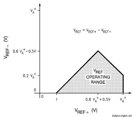
FIGURE 19. V_{\text{REF}} Operating Range
