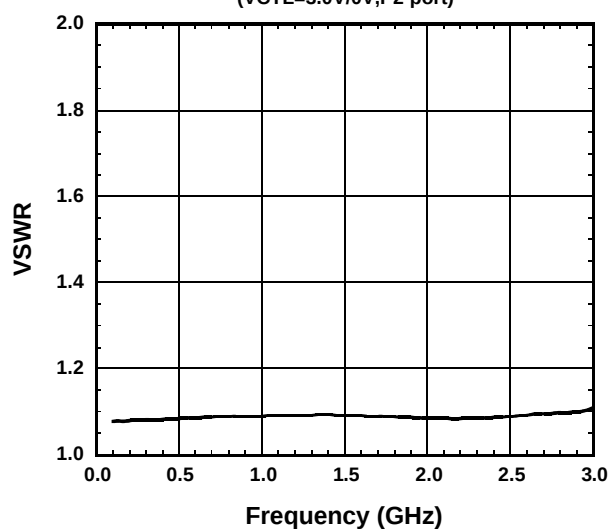
PC-P2 VSWR vs. Frequency
