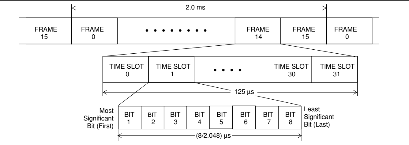
Figure 30 - PCM 30 Format
