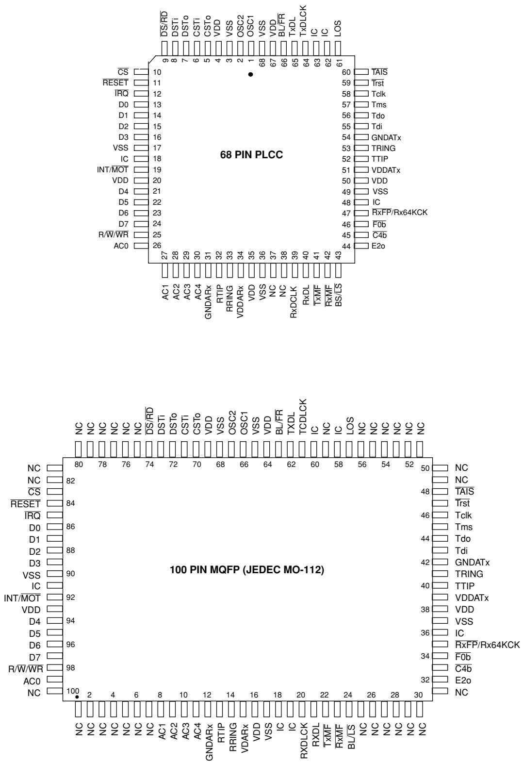
Figure 2 - Pin Connections
